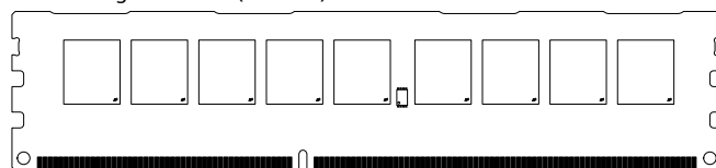
Figure 1: 240-Pin UDIMM (MO-269 R/C E)
