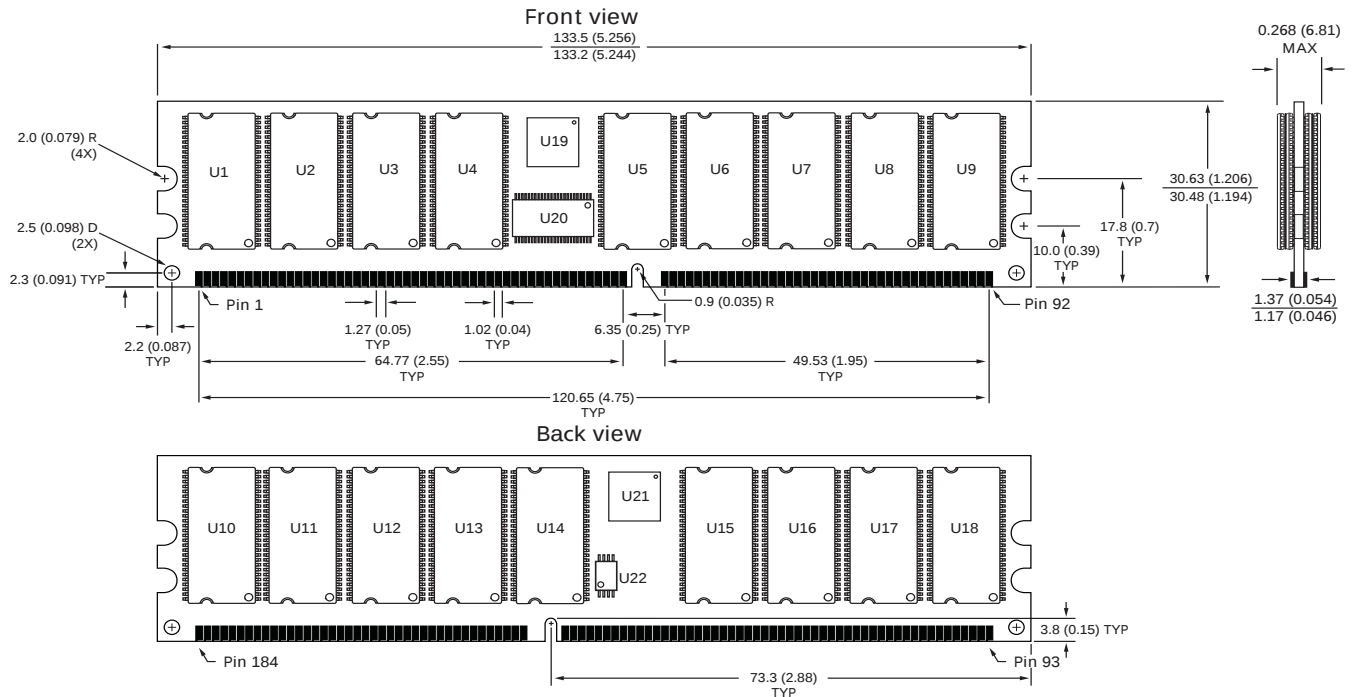
Figure 6: 184-Pin DDR RDIMM – Low Profile, 43.18mm (1.2in)
