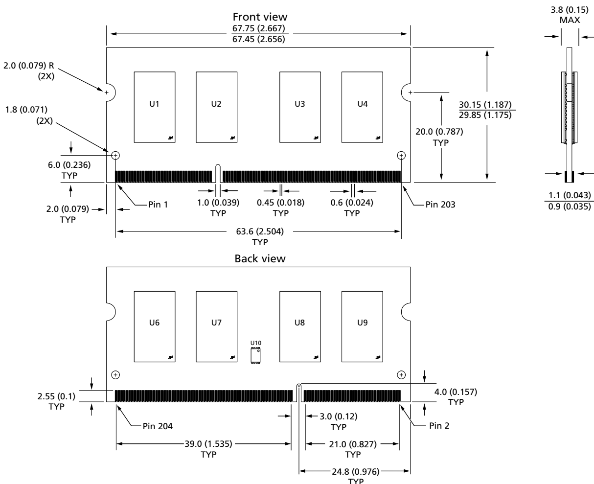
Figure 3: 204-Pin DDR3 SODIMM
