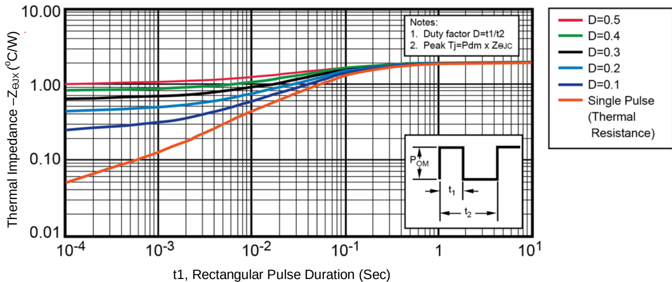
FIGURE 2 Thermal Impedance
