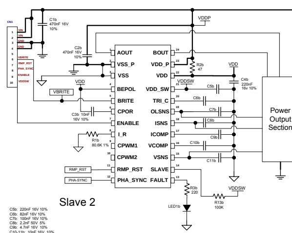
Figure 2 – Schematic Modules Connected as a Master and Slave
