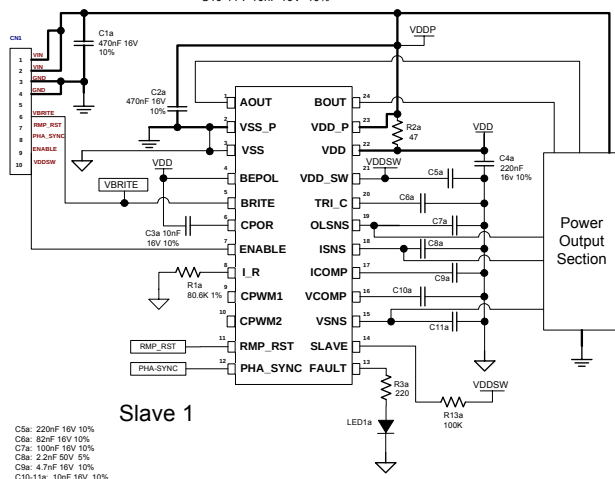
Figure 2 – Schematic Modules Connected as a Master and Slave
