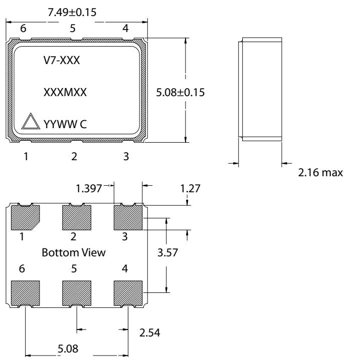
Figure 5 Optional Package Outline Drawing
