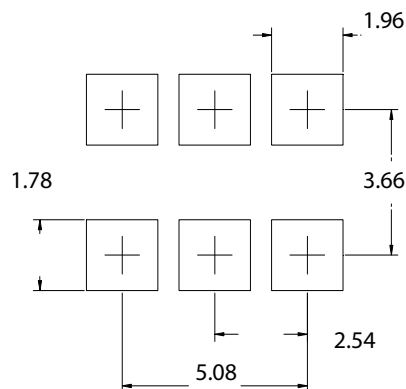
Figure 6 Pad Layout
