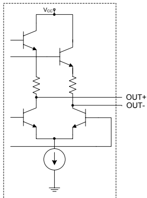
Figure 10 Standard LVDS Output Configuration
