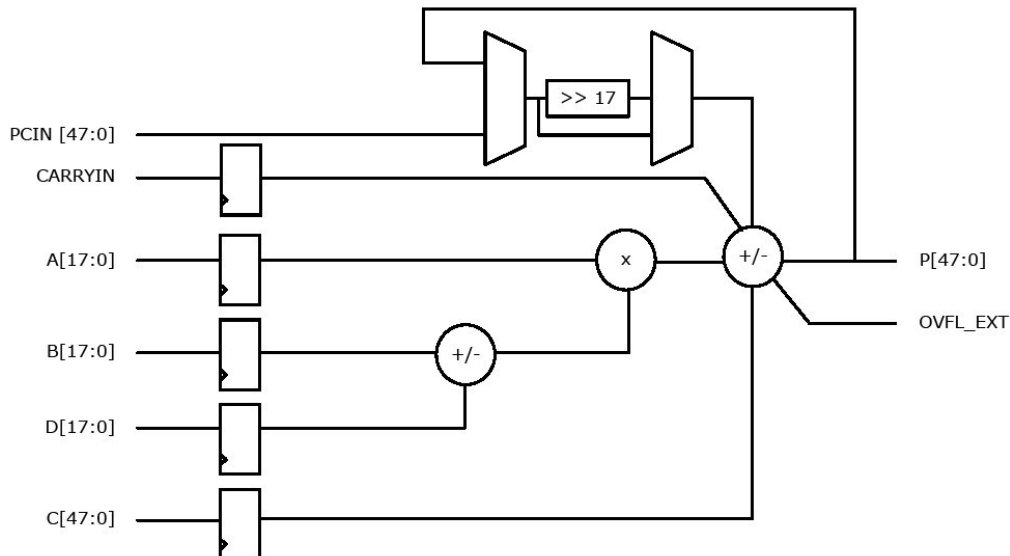
Figure 3 • Math Block
