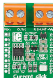
Current click™
