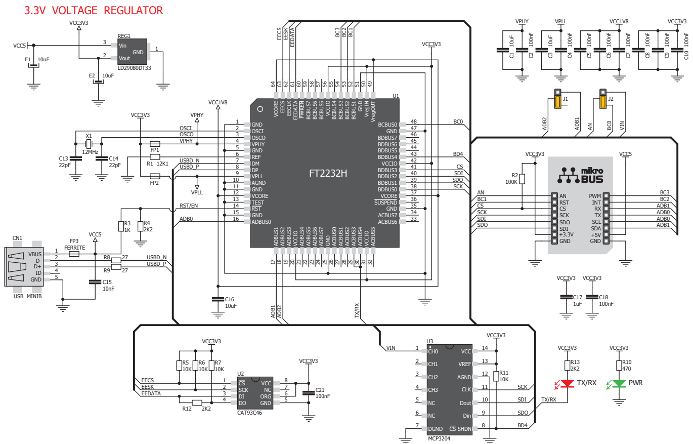
Figure 1: Click USB adapter schematic
