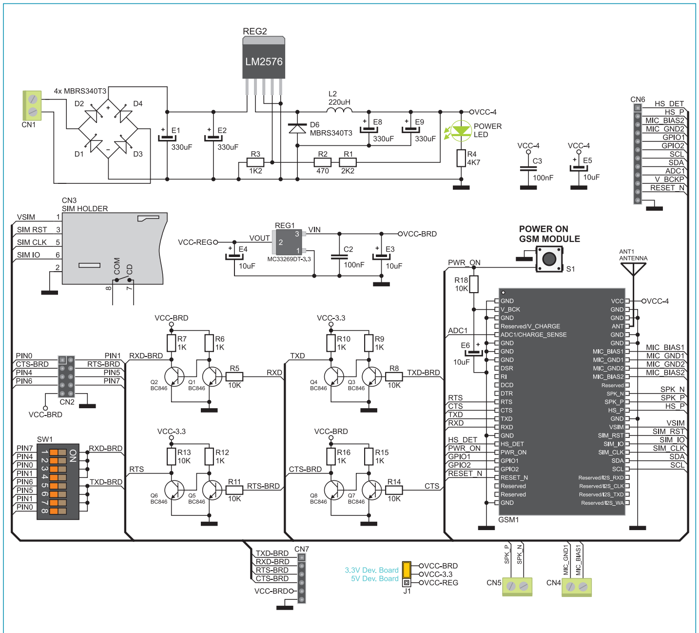
Figure 4: SmartG100 connection schematics
