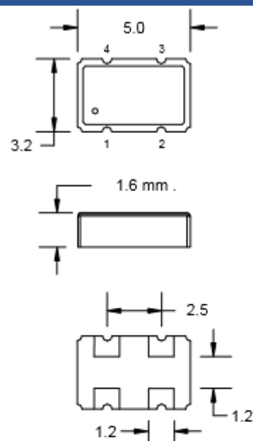
Recommended Pad Layout
