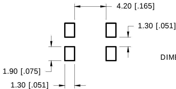
SUGGESTED LAND PATTERN
