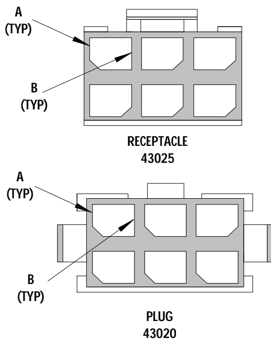
Figure 1 CONNECTOR PATTERN
