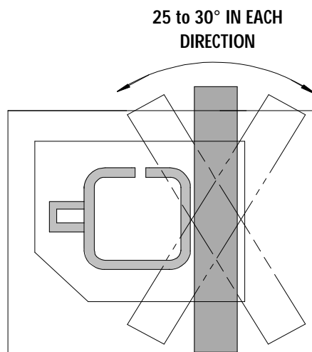
Figure 2 ROTATING TOOL
