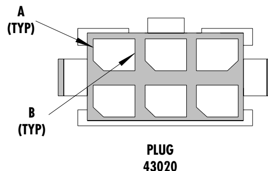
Figure 1 CONNECTOR PATTERN
