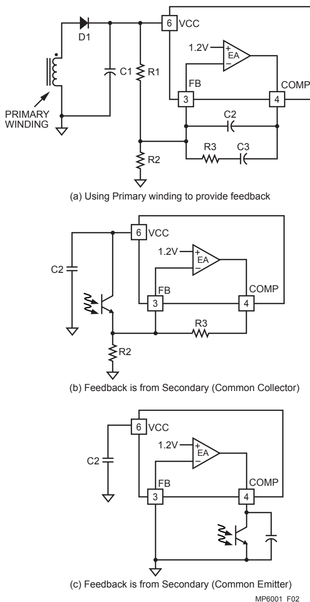
Figure 2—Error Amplifier Configurations
