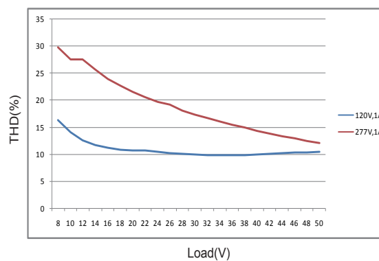
Current Total Harmonic Curve
