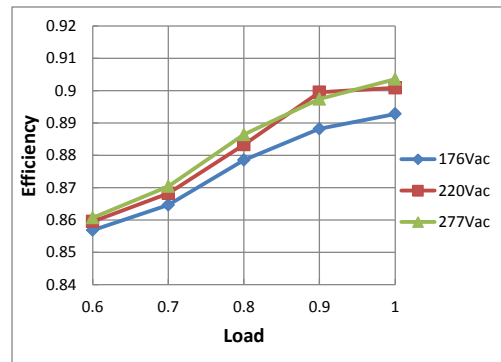
Efficiency VS. Load Curve
