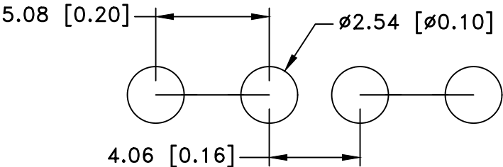
MOUNTING DETAIL
