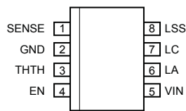
Pin-out Diagram
