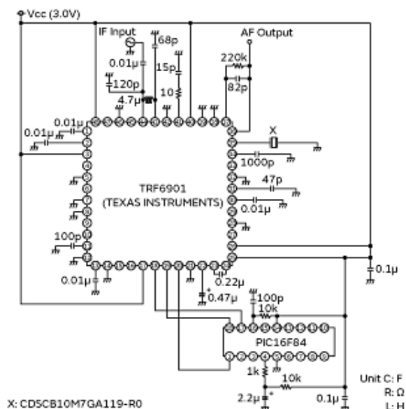
Measurement Circuit
