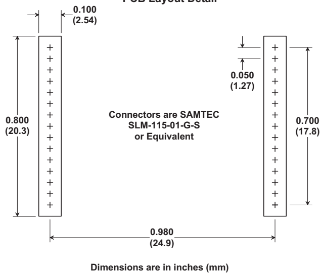
DNT90MP Interface Connector PCB Layout Detail
