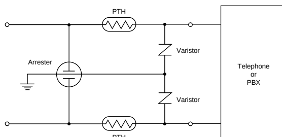
(5) Telecommunication Circuit
