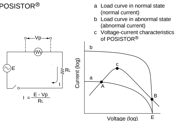
Load Curve of Circuit and Voltage - Current Characteristics of POSISTOR®
