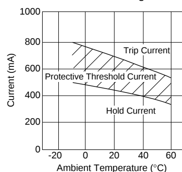
Protective Threshold Current Range
