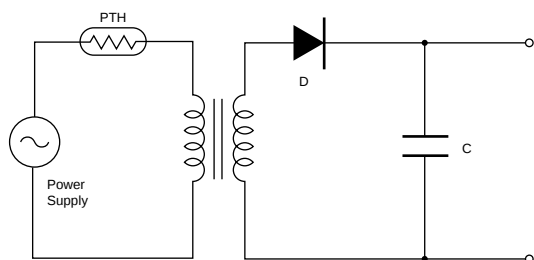
(1) Transformer Protection Circuit 1)
