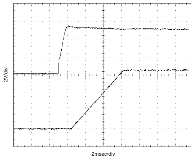
Power-Up From V IN
