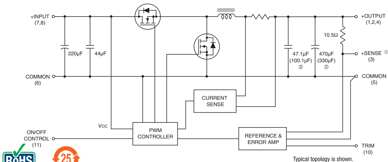
Figure 1. Simplified Schematic
