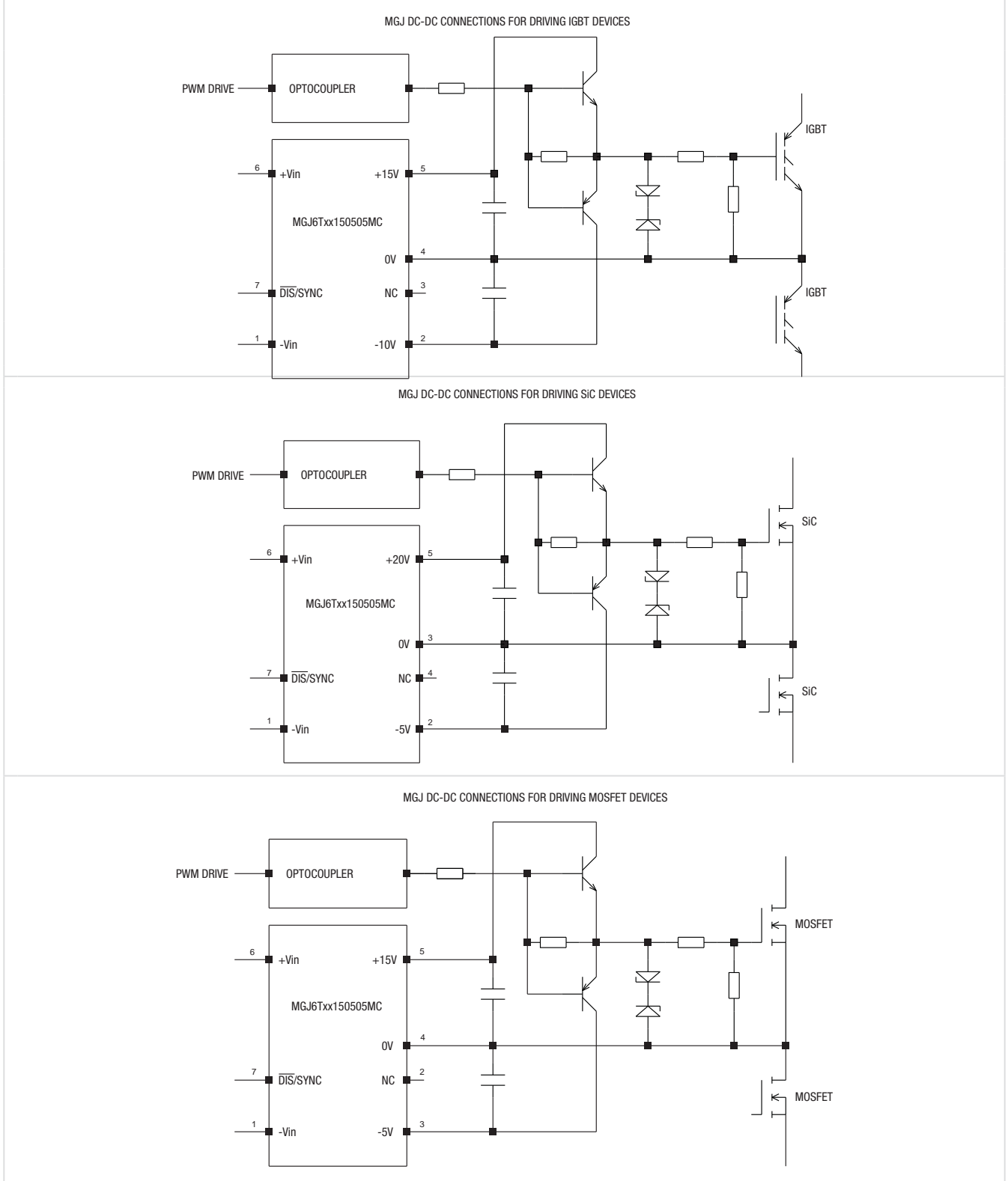
Schematic for driving IGBT, SiC & MOSFET (DIP)
