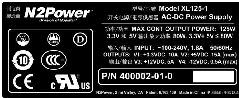
Figure 4-1 Sample XL160 Label
