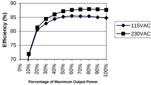
XL160-19, -24, -28, -30 [CS] Efficiency
