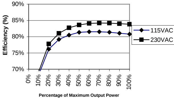
XL160-7 Efficiency
