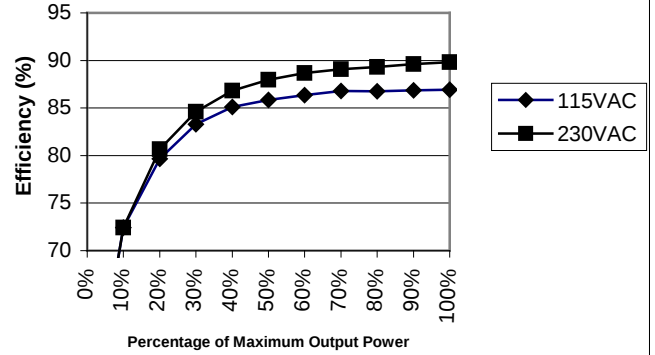
XL160-48, -51, -54, -56 [CS] Efficiency
