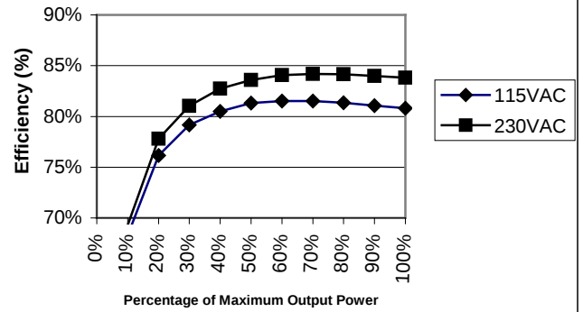
XL160-8, -11 Efficiency
