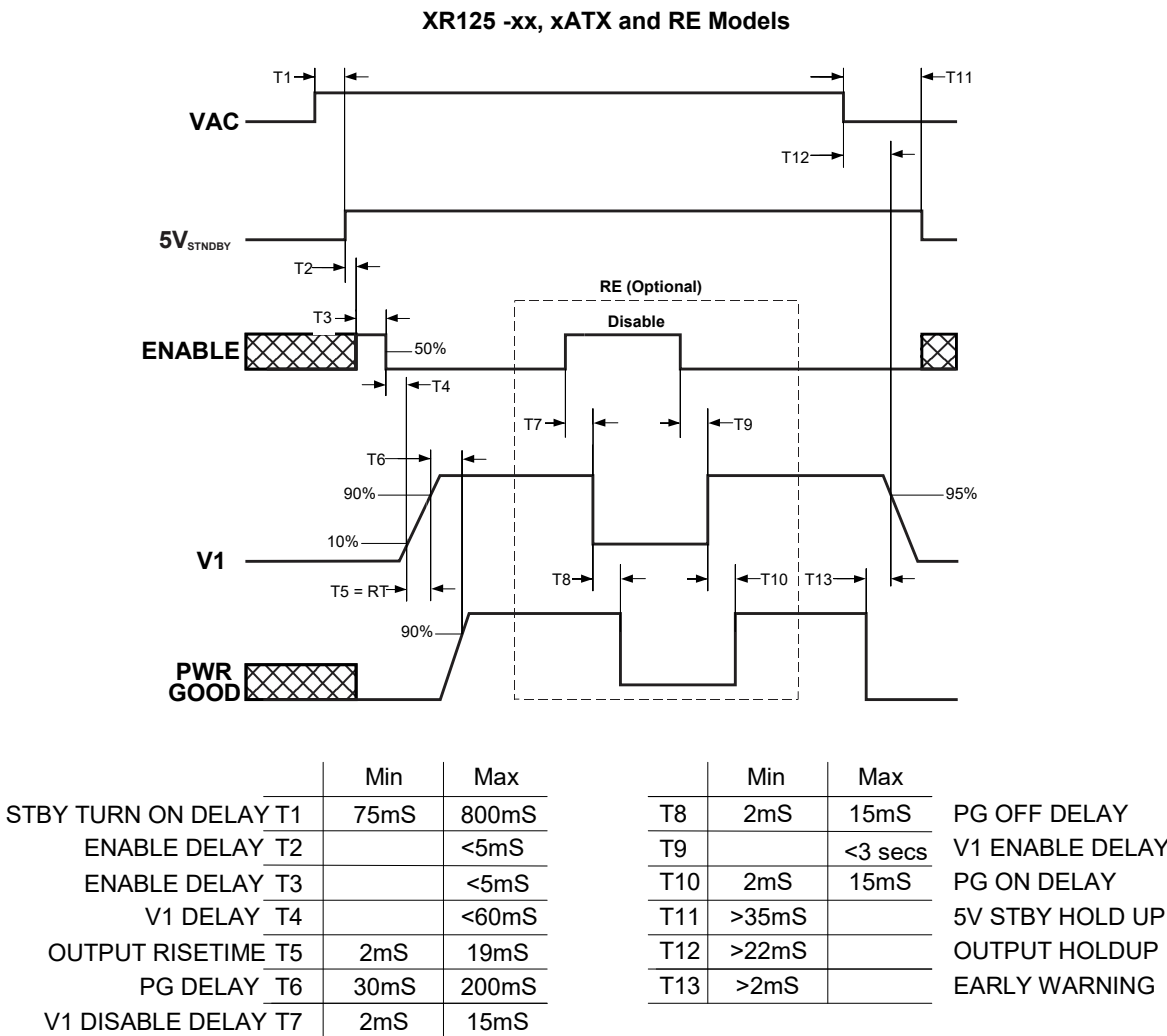
Figure 6-1 XR125 Timing Diagram
