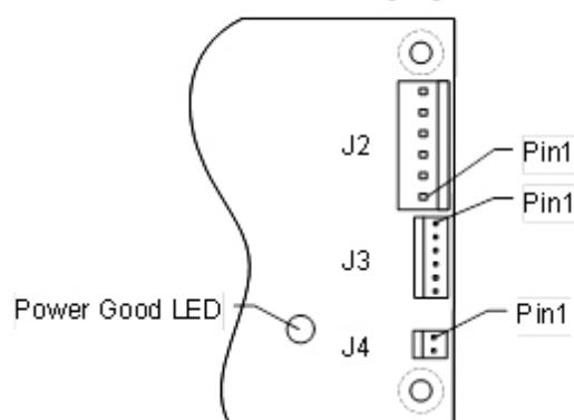
XR125-xx [CS]
