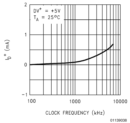
Digital Supply Current ( I_{D+} ) vs. Clock Frequency
