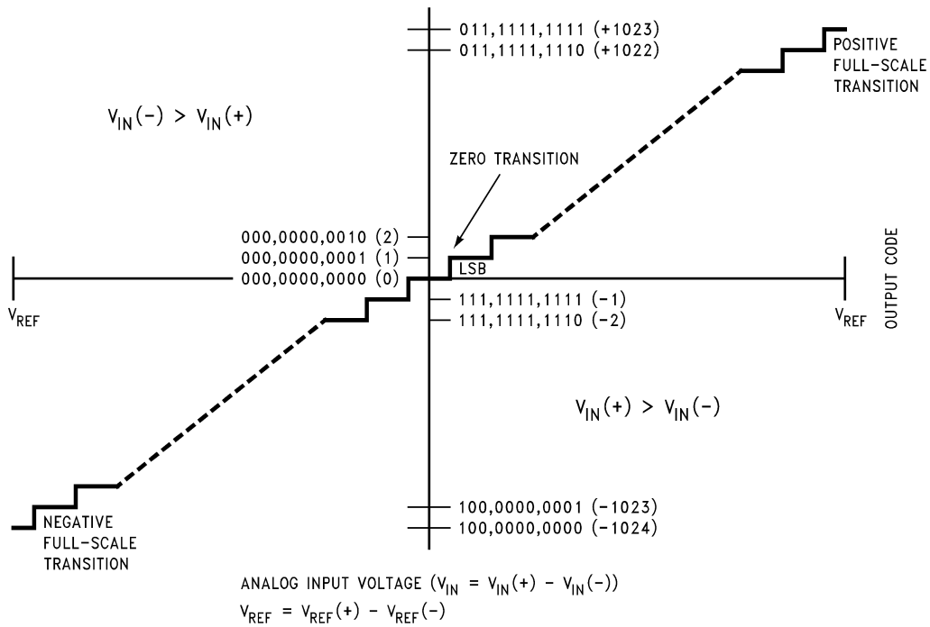
FIGURE 1. Transfer Characteristic
