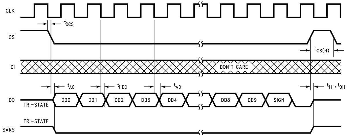
FIGURE 5. Delayed DO Timing
