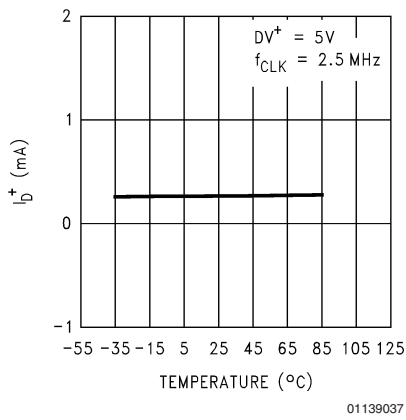
Digital Supply Current ( I_{D+} ) vs. Temperature
