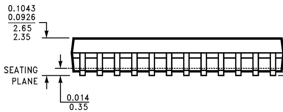
Order Number ADC10738CIWM NS Package Number M24B
