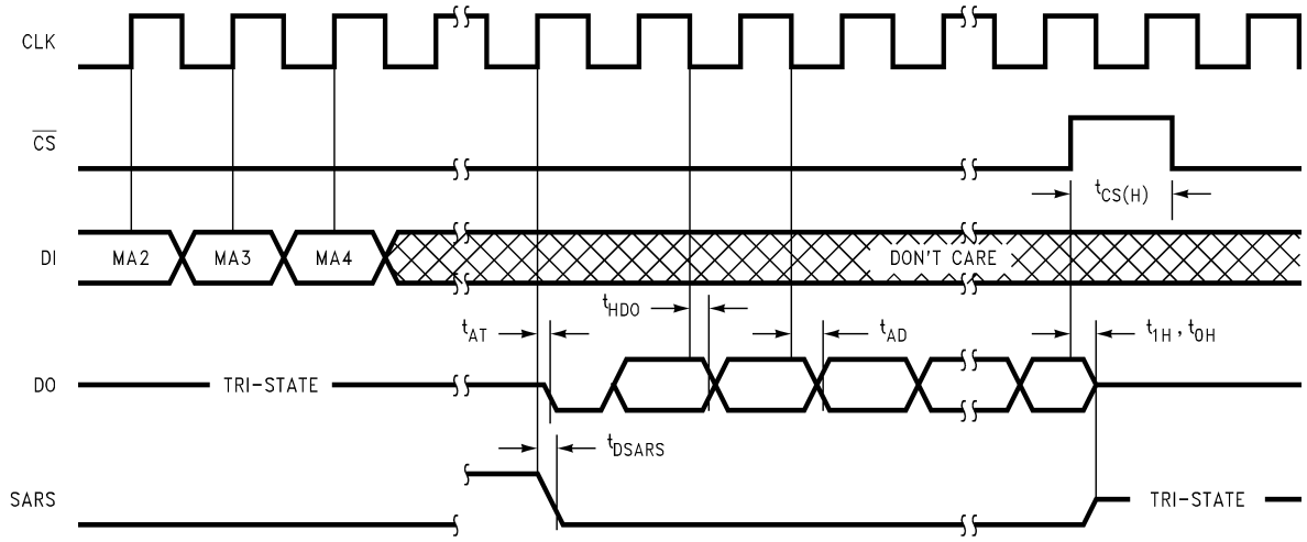
FIGURE 4. DO Timing
