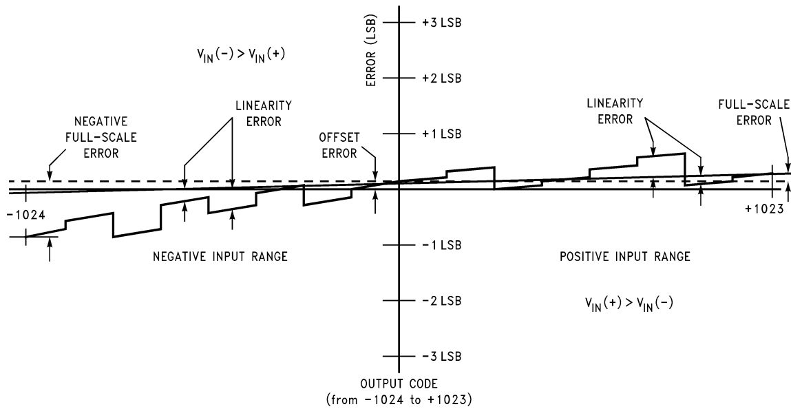
FIGURE 2. Simplified Error Curve vs. Output Code
