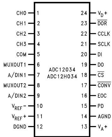
24-Pin Wide Body SO, DIP, SSOP-EIAJ Packages
