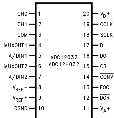
20-Pin Wide Body SO Packages
