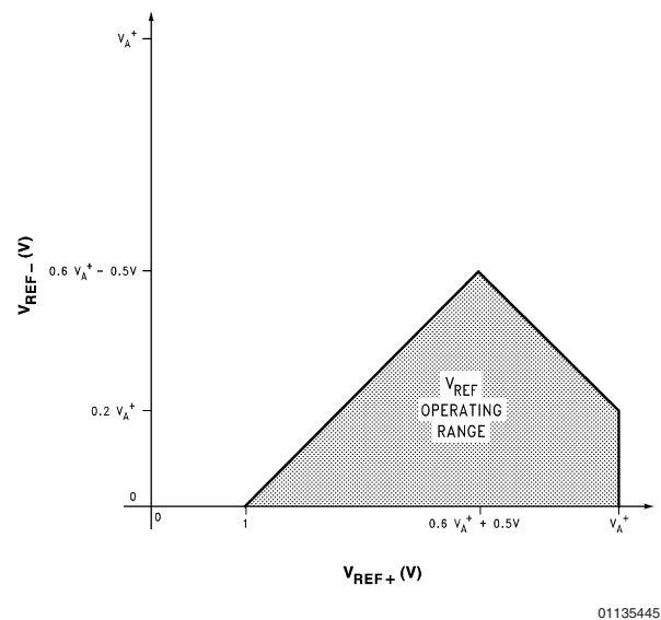
FIGURE 17. V_{REF} Operating Range
