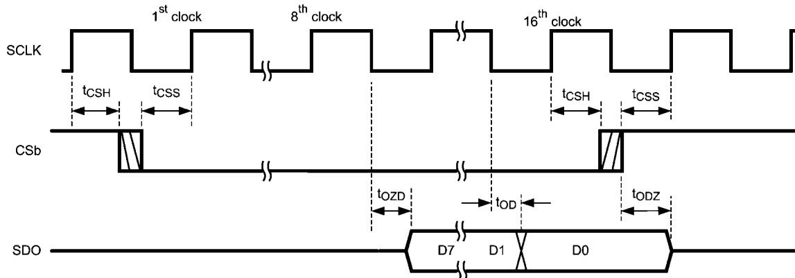
FIGURE 14. Read Timing
