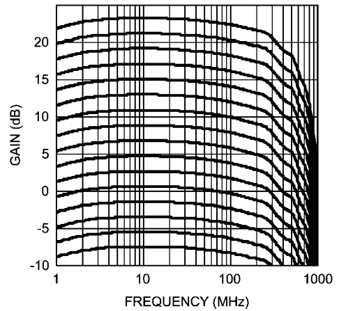
Frequency Response 2dB Gain Steps Transformer Coupled
