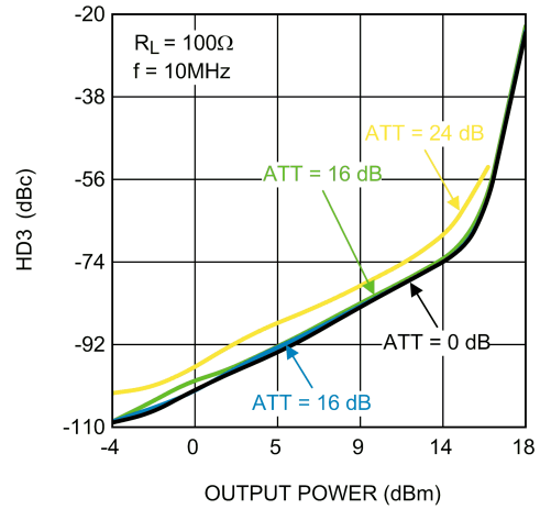
Third Order Harmonic Distortion at 10 MHz
