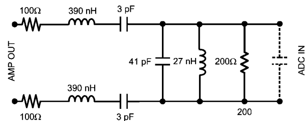
FIGURE 18. Bandpass Filter Center Frequency is 140 MHz with a 20 MHz Bandwidth Designed for 200Ω Impedance
