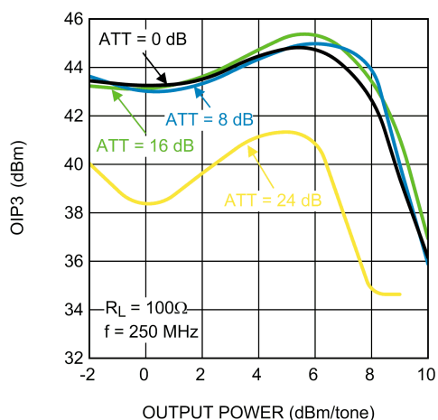
Third Order Intercept Point at Various Attenuator Settings f = 250 \text{ MHz}
