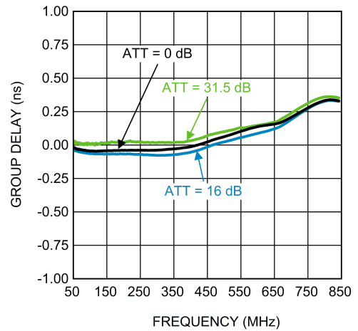
Group Delay
