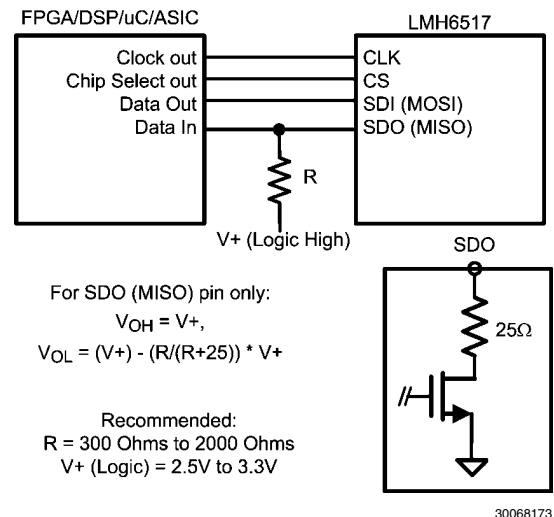
FIGURE 12. SDO Pin External Bias Resistor Configuration
