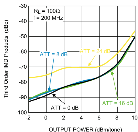
Third Order Intermodulation at Various Attenuator Settings f = 200 \text{ MHz}
