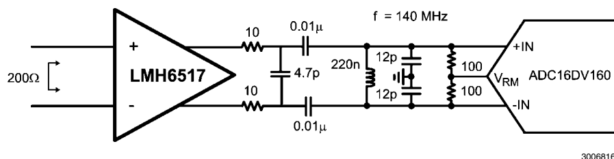
FIGURE 6. Output Configuration
