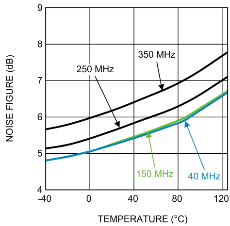
Noise Figure vs. Temperature
