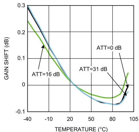
Gain Shift vs Temperature
