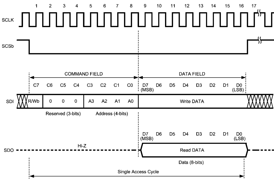
FIGURE 13. Serial Interface Protocol (SPI compatible)
