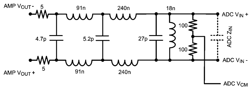
FIGURE 20. Impedance Transforming Filter 25 Ω Input 200 Ω Output, 210 MHz Center Frequency
