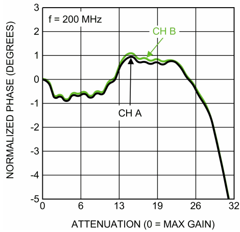
Phase Shift vs Attenuator Setting
