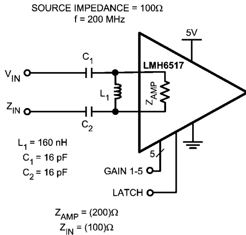
FIGURE 4. Differential 200Ω LC Conversion Circuit
