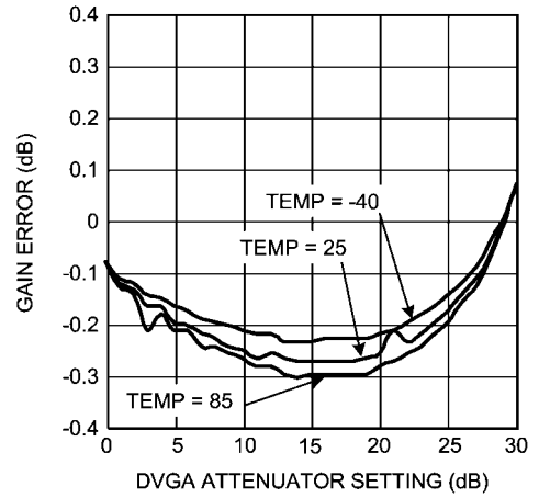
Cumulative Gain Error over Temperature
