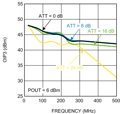
Third Order Intercept Point vs Frequency
