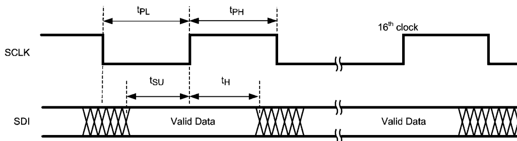
FIGURE 15. Write Timing Data Written to SDI Pin
