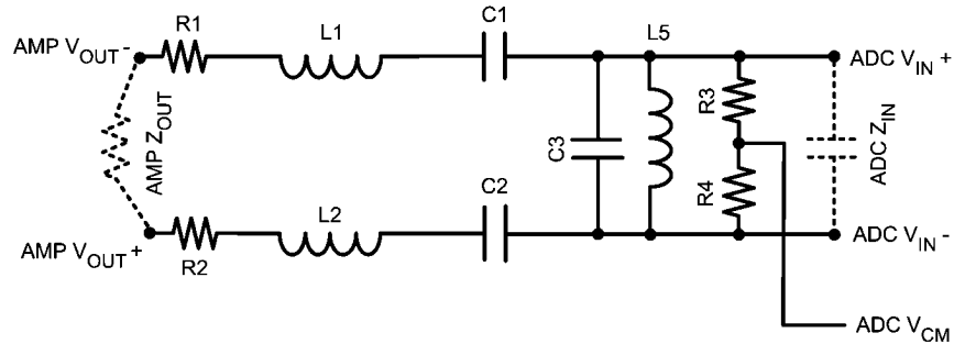
FIGURE 19. Sample Filter
