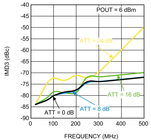
Third Order Intermodulation Products vs Frequency
