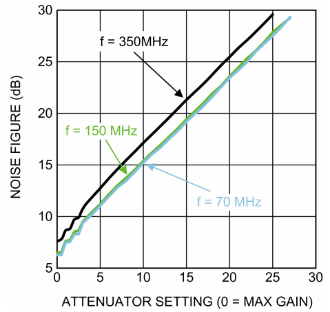
Noise Figure vs Attenuator Setting
