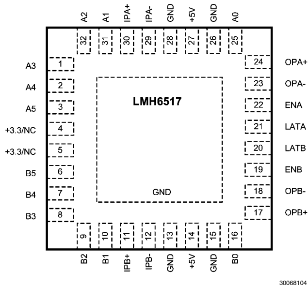
FIGURE 7. Pin Functions for Parallel Mode
