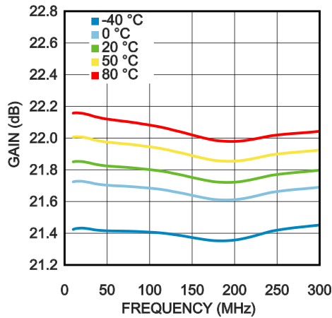
Gain Flatness over Temperature
