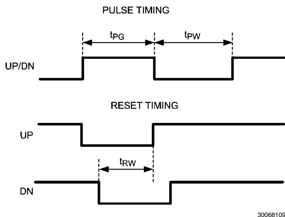
FIGURE 17. Pulse Mode Timing
