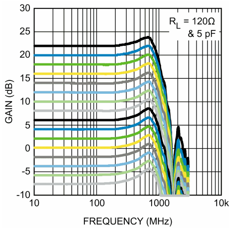
Frequency Response 2dB Gain Steps
