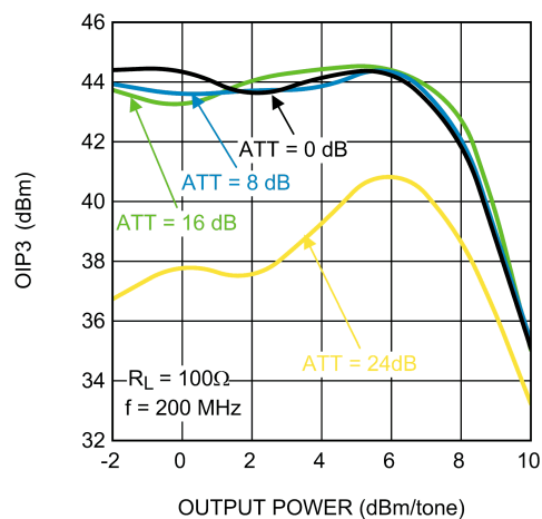
Third Order Intercept Point at Various Attenuator Settings f = 200 \text{ MHz}
