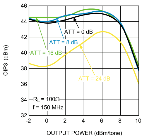
Third Order Intercept Point at Various Attenuator Settings f = 150 \text{ MHz}
