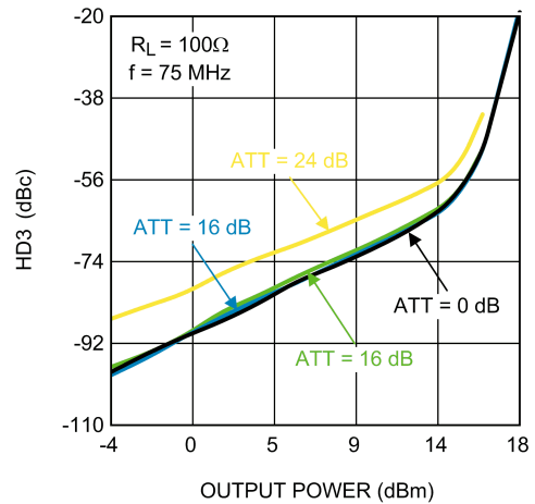
Third Order Harmonic Distortion at 75 MHz
