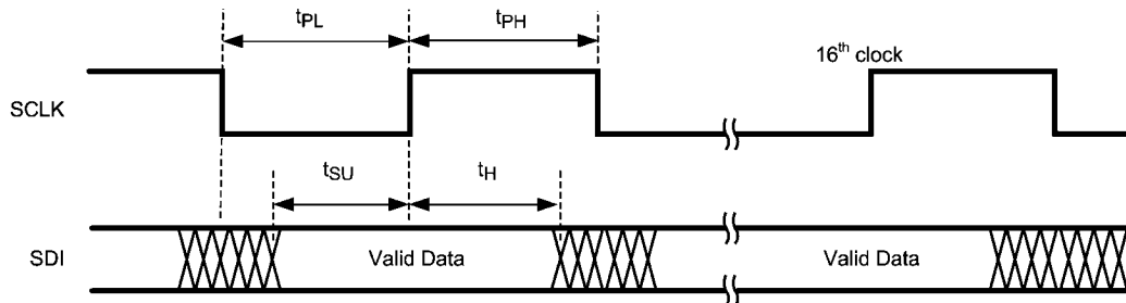
FIGURE 15. Write Timing Data Written to SDI Pin
