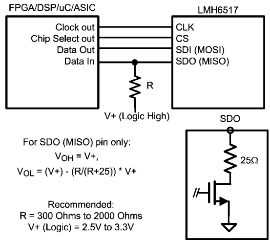
FIGURE 12. SDO Pin External Bias Resistor Configuration
