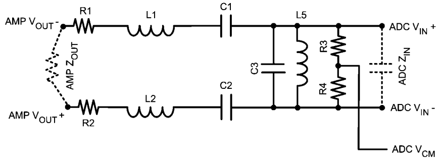
FIGURE 19. Sample Filter
