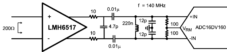
FIGURE 6. Output Configuration
