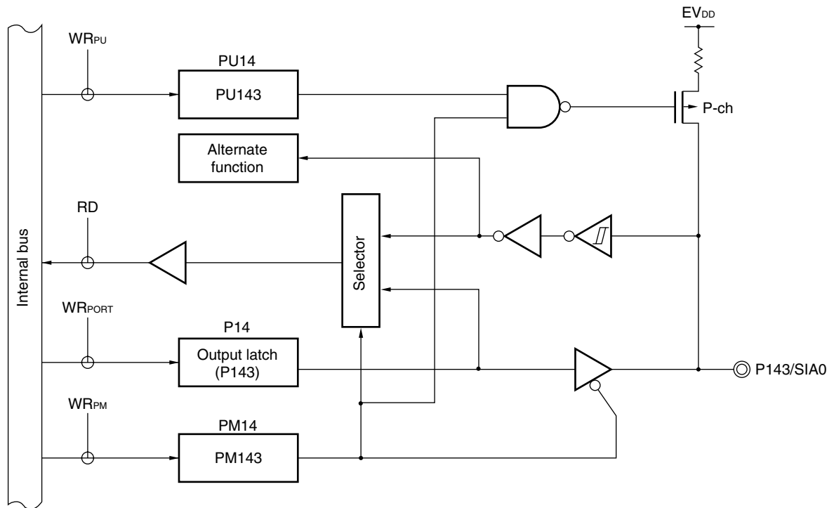
Figure 5-26. Block Diagram of P143
