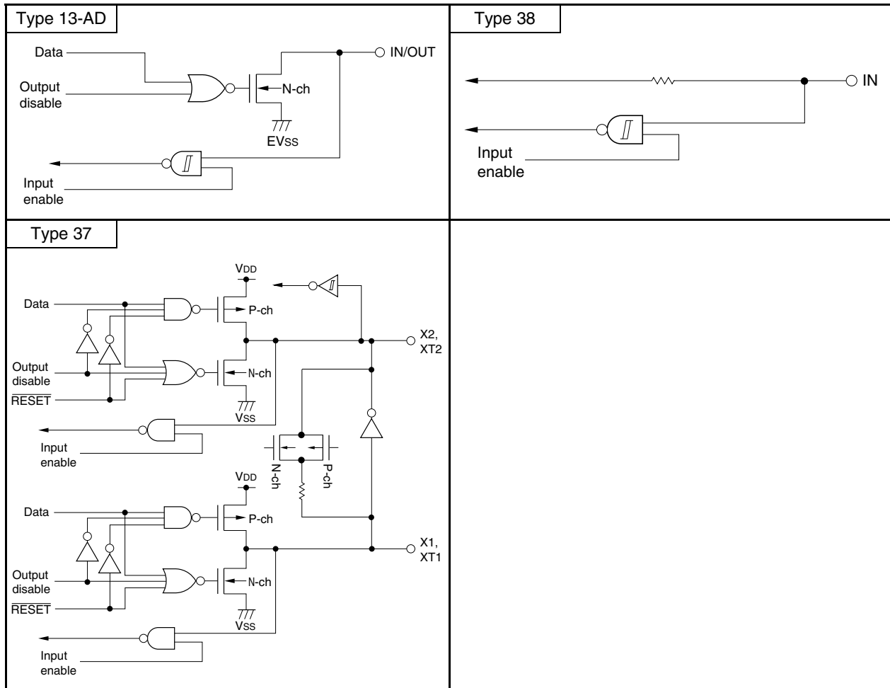
Figure 2-1. Pin I/O Circuit List (2/2)
