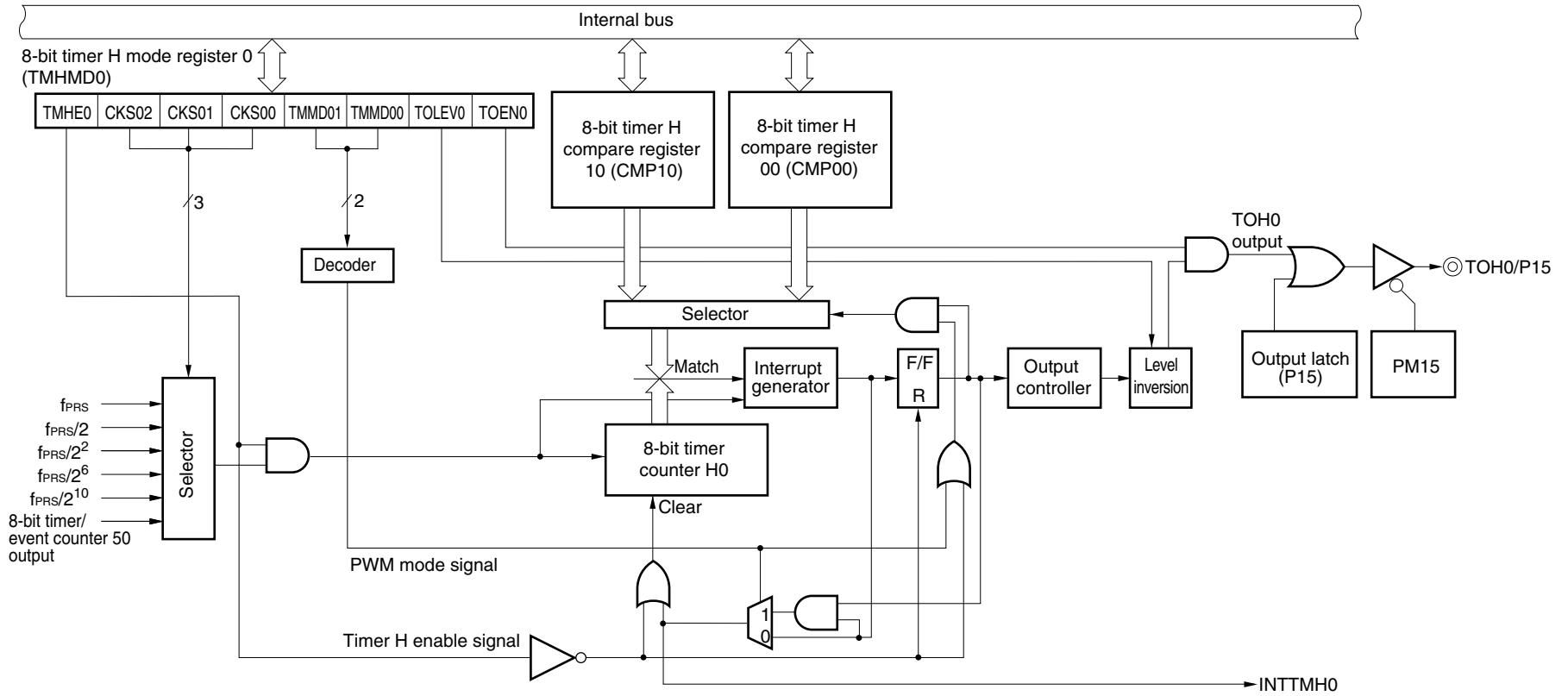
&lt;R&gt; Figure 9-1. Block Diagram of 8-Bit Timer H0
