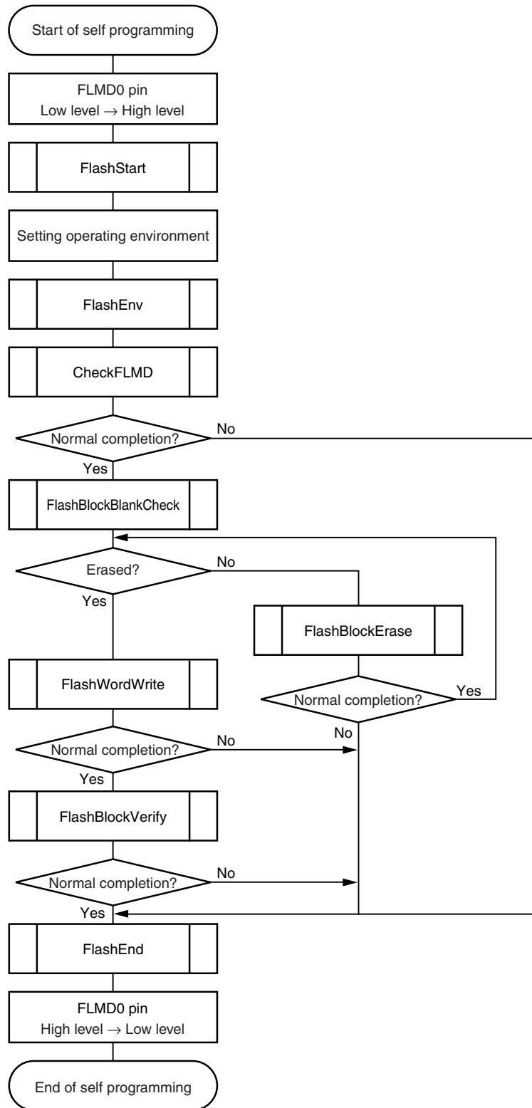
Figure 27-16. Flow of Self Programming (Rewriting Flash Memory)
