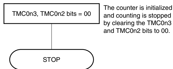
&lt;3&gt; Count operation stop flow
