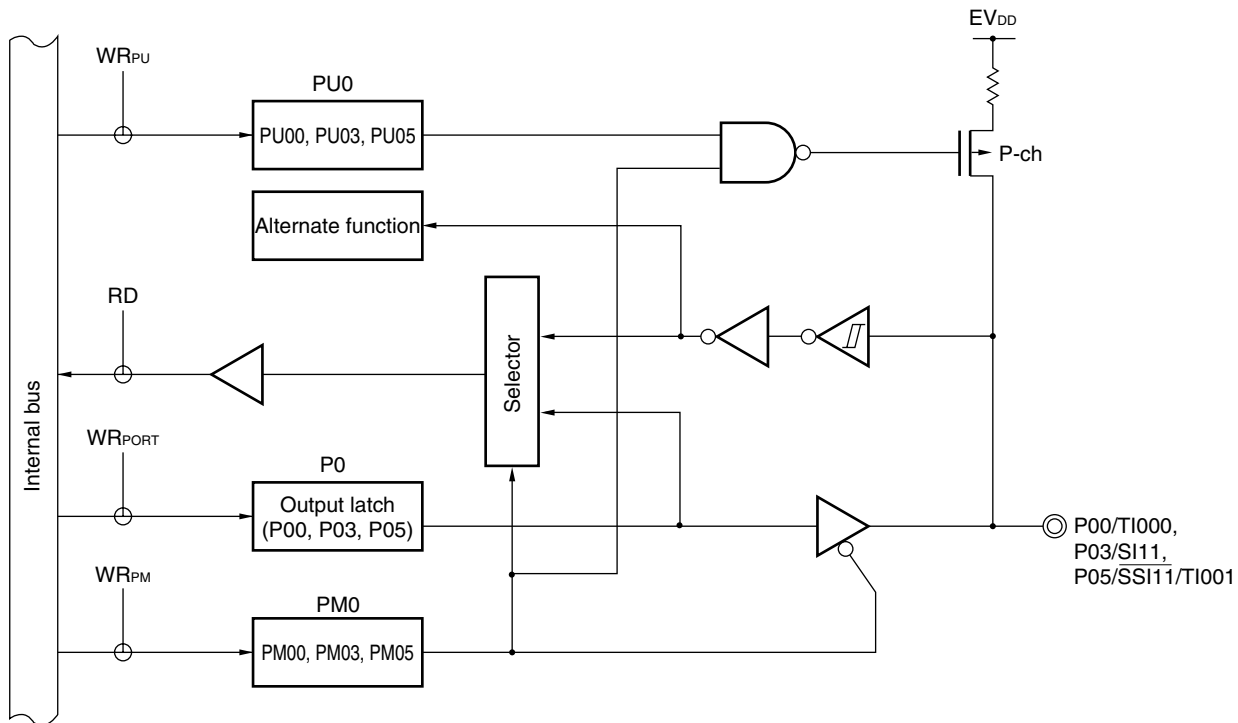
Figure 5-2. Block Diagram of P00, P03, and P05
