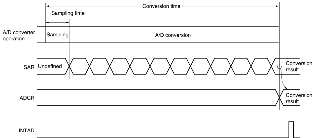
Figure 13-11. Basic Operation of A/D Converter
