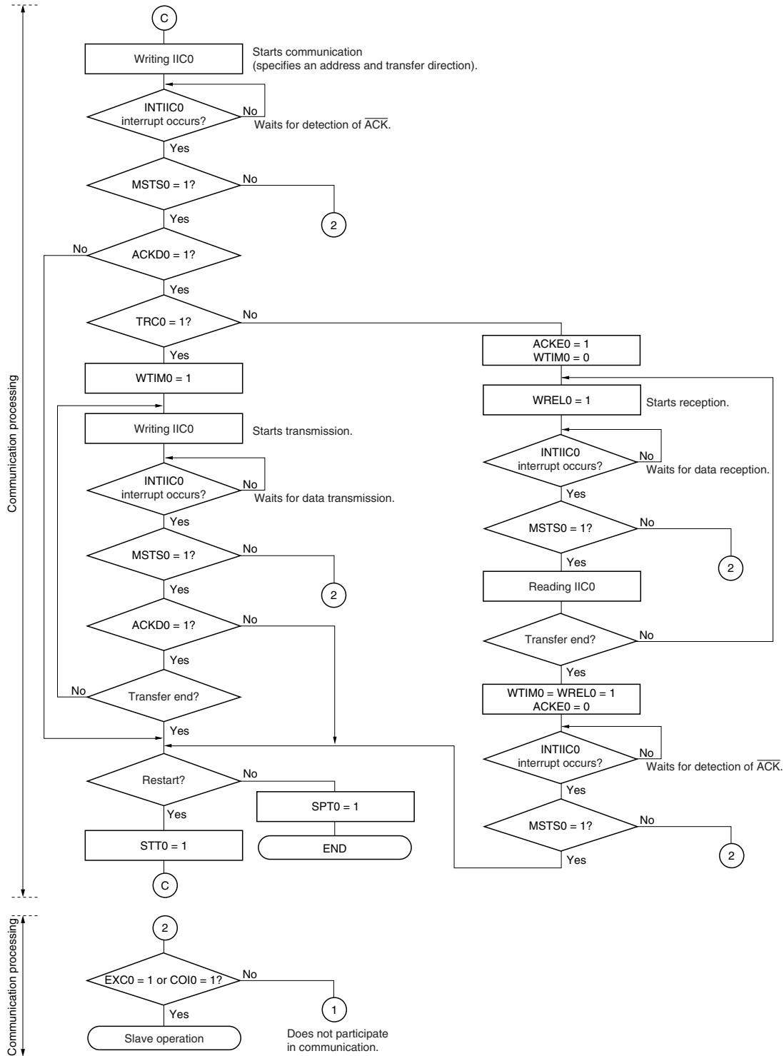
Figure 18-24. Master Operation in Multi-Master System (3/3)
