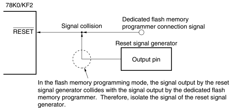
Figure 27-11. Signal Collision ( \overline{\text{RESET}} Pin)
