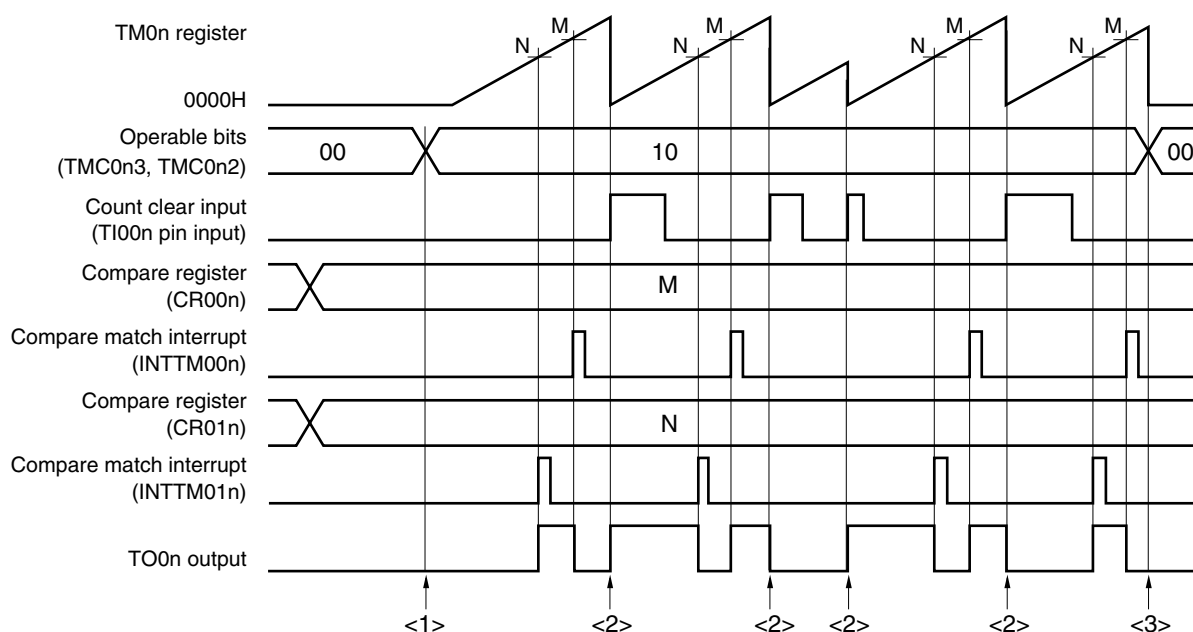
<R> Figure 7-36. Example of Software Processing in Clear & Start Mode Entered by TI00n Pin Valid Edge Input
