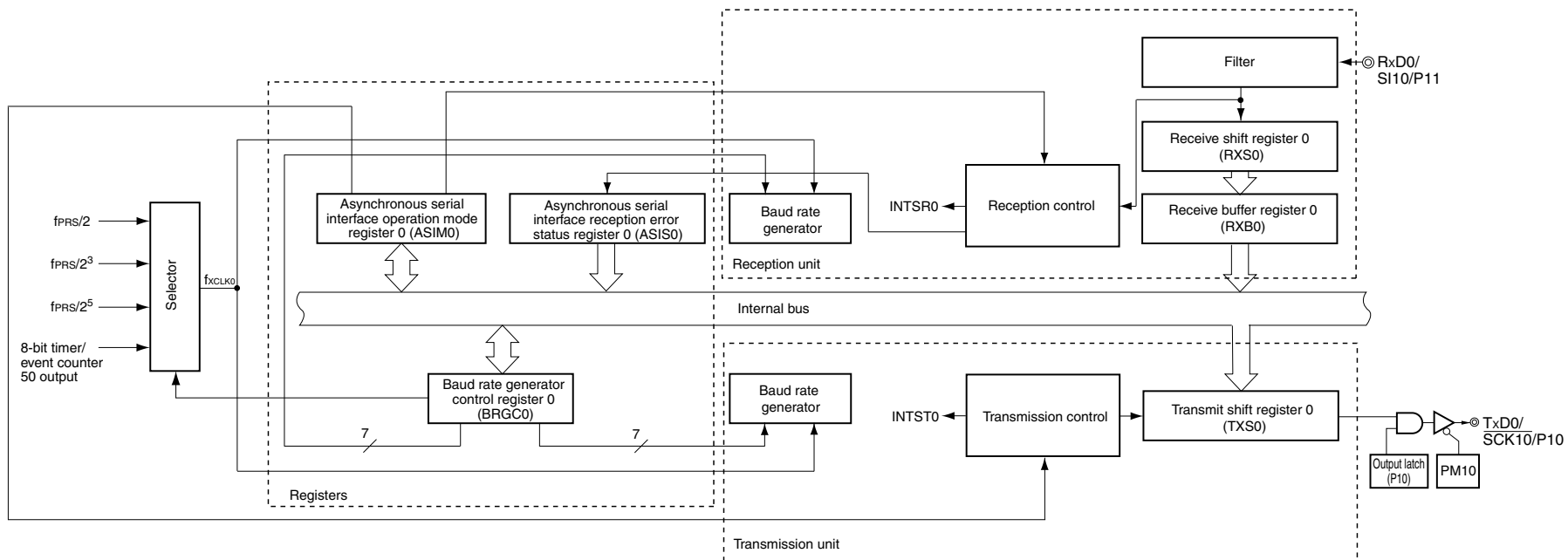
<R> Figure 14-1. Block Diagram of Serial Interface UART0
