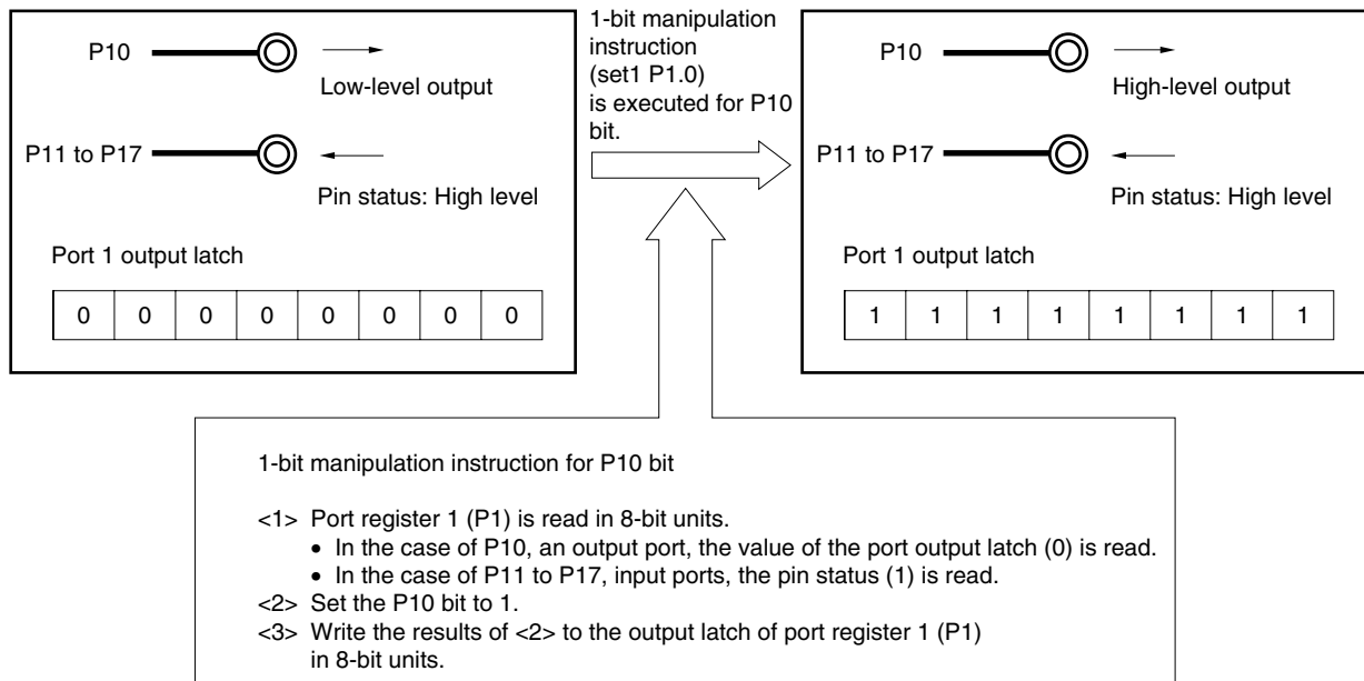
Figure 5-32. Bit Manipulation Instruction (P10)
