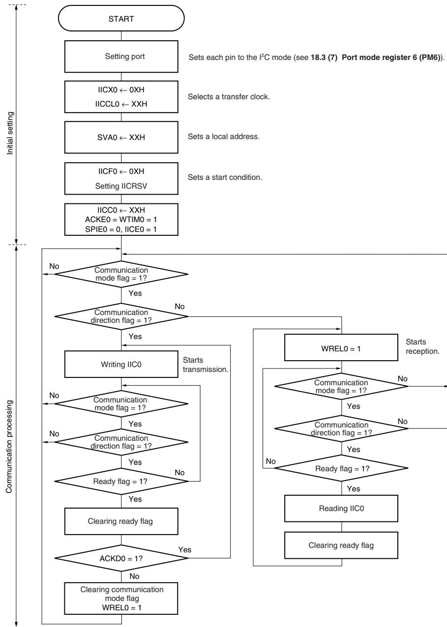
Figure 18-25. Slave Operation Flowchart (1)
