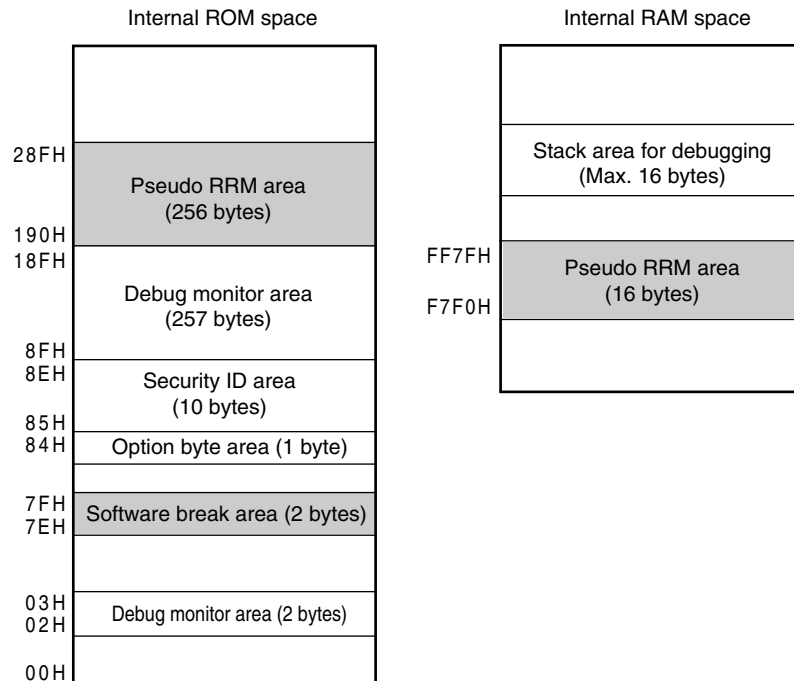
Figure 28-4. Reserved Area Used by QB-78K0MINI and QB-MINI2
