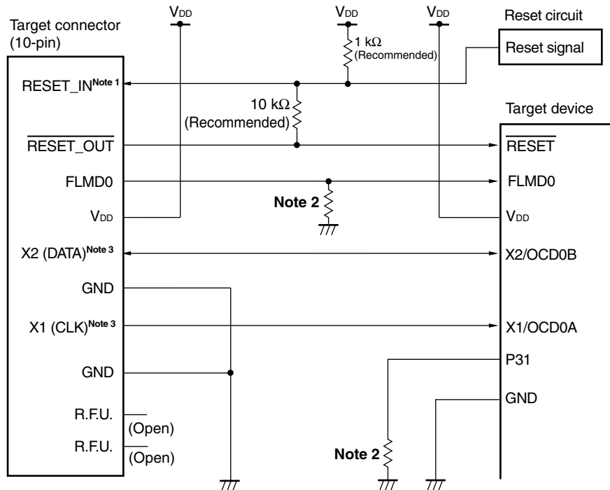
Figure 28-1. Connection Example of QB-78K0MINI or QB-MINI2 and \mu PD78F0547D (When OCD0A/X1 and OCD0B/X2 Are Used)
