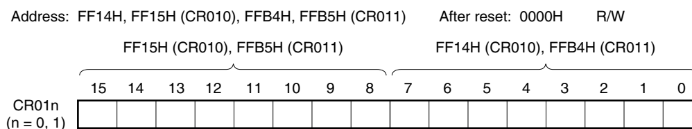
Figure 7-5. Format of 16-Bit Timer Capture/Compare Register 01n (CR01n)
