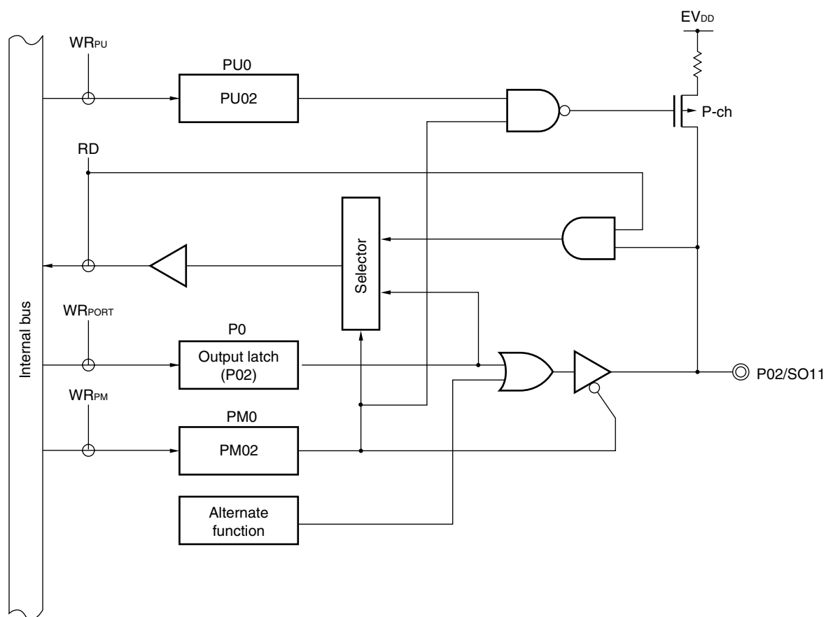
Figure 5-4. Block Diagram of P02
