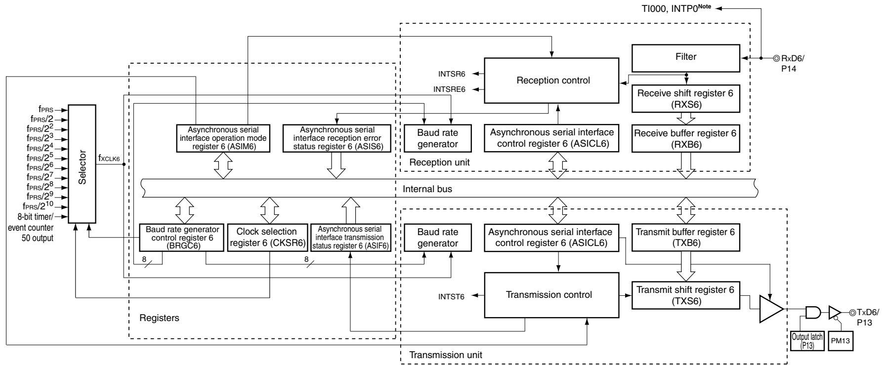
<R> Figure 15-4. Block Diagram of Serial Interface UART6
