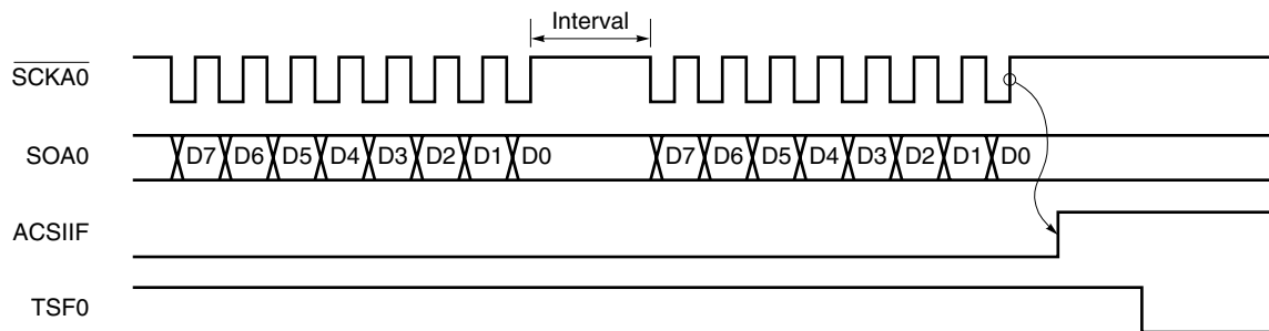
Figure 17-17. Example of Automatic Transmission Mode Operation Timing
