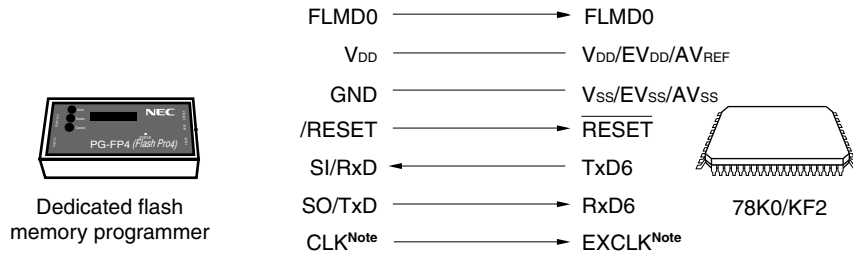
Figure 27-7. Communication with Dedicated Flash memory programmer (UART6)
