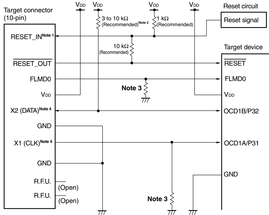
Figure 28-2. Connection Example of QB-78K0MINI or QB-MINI2 and \mu PD78F0547D (When OCD1A/P31 and OCD1B/P32 Are Used)
