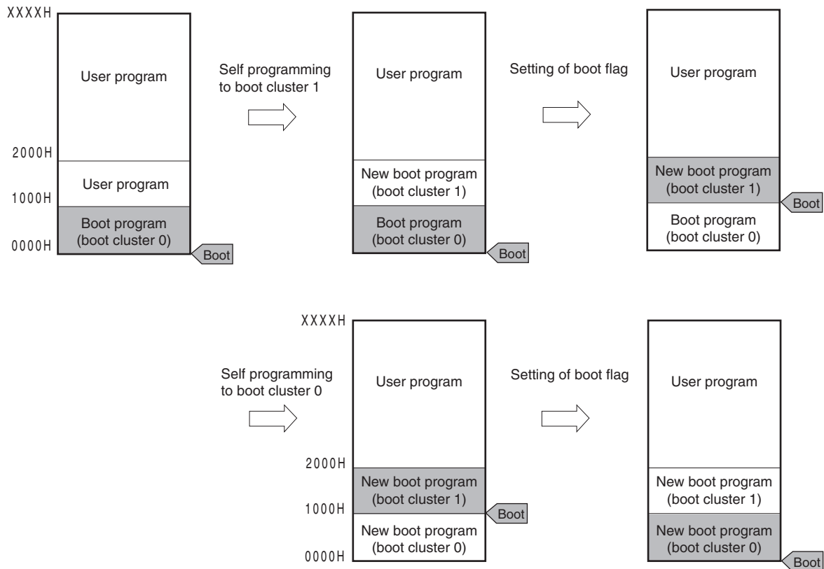
<R> Figure 27-17. Boot Swap Function
