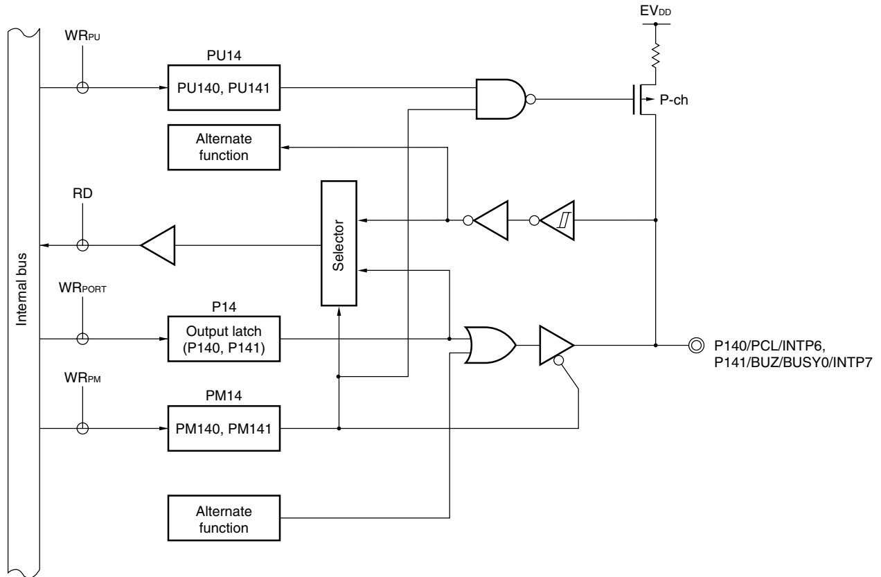
Figure 5-24. Block Diagram of P140 and P141
