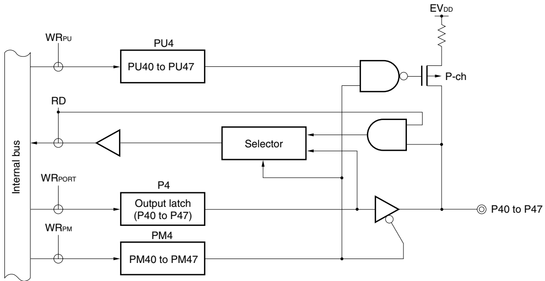
Figure 5-14. Block Diagram of P40 to P47
