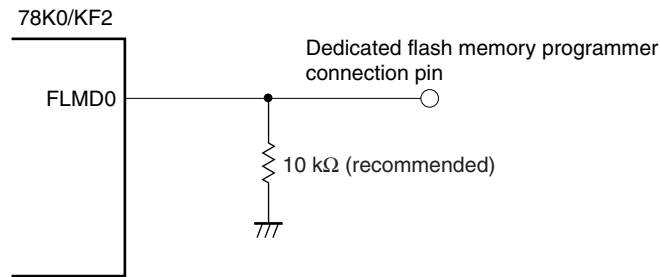
Figure 27-8. FLMD0 Pin Connection Example
