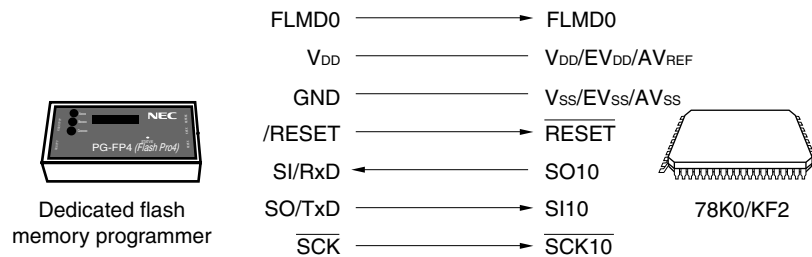
Figure 27-6. Communication with Dedicated Flash memory programmer (CSI10)
