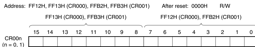
Figure 7-4. Format of 16-Bit Timer Capture/Compare Register 00n (CR00n)
