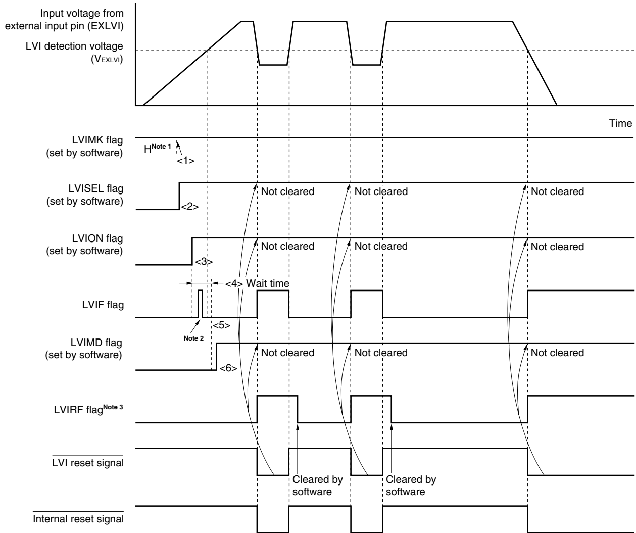
Figure 25-6. Timing of Low-Voltage Detector Internal Reset Signal Generation (Detects Level of Input Voltage from External Input Pin (EXLVI))
