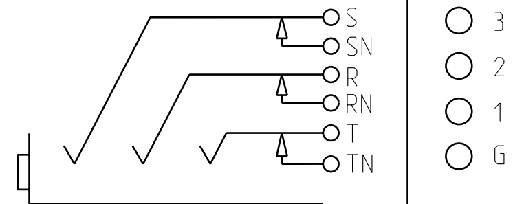
JACK- NORMALLING
