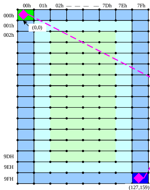
GRAM size(128x160x18-bits)
