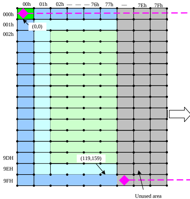
GRAM size(120x160x18-bits)
