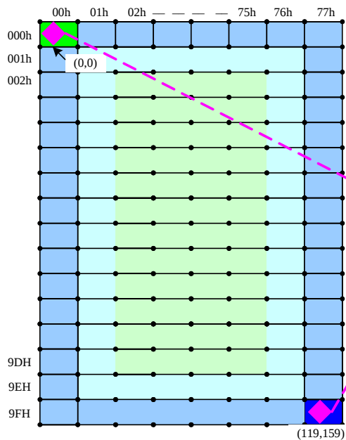
GRAM size(120x160x18-bits)
