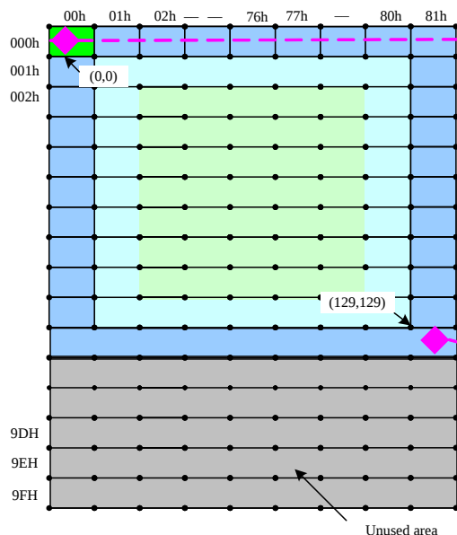
GRAM size(130x130x18-bits)
