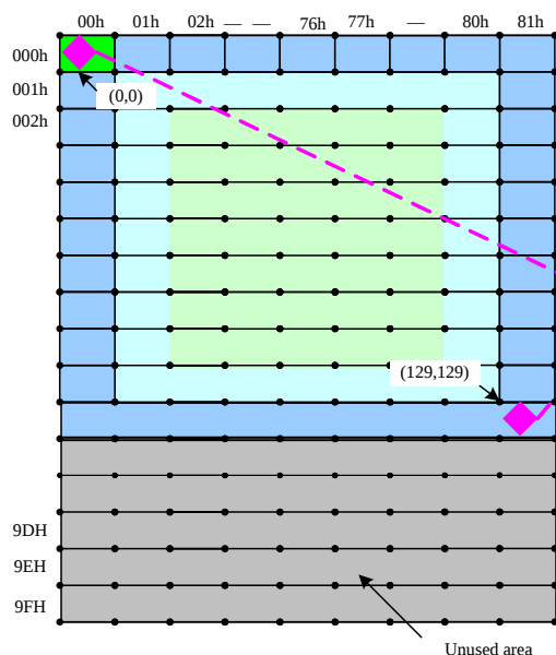
GRAM size(130x130x18-bits)
