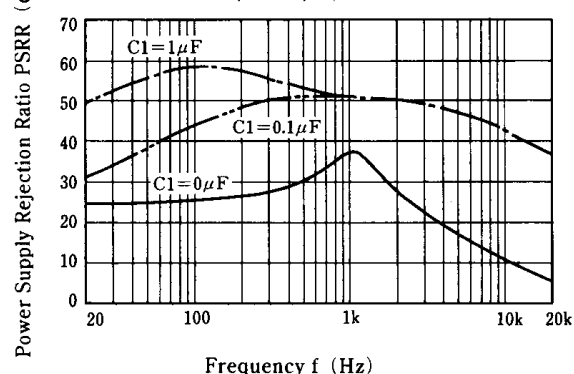
Power Supply Rejection Ratio vs. Frequency ( C_2 = 5\mu\text{F} )
