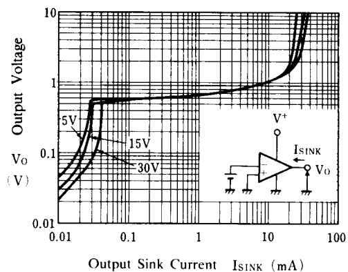
Output Sink Current
