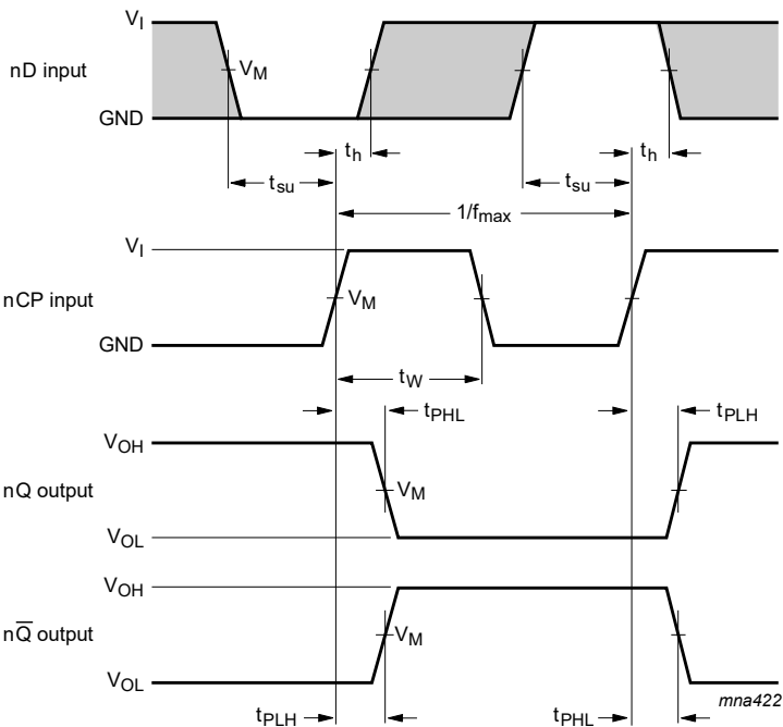
Measurement points are given in Table 8. The shaded areas indicate when the input is permitted to change for predictable output performance. V_{OL} and V_{OH} are typical voltage output levels that occur with the output load.
