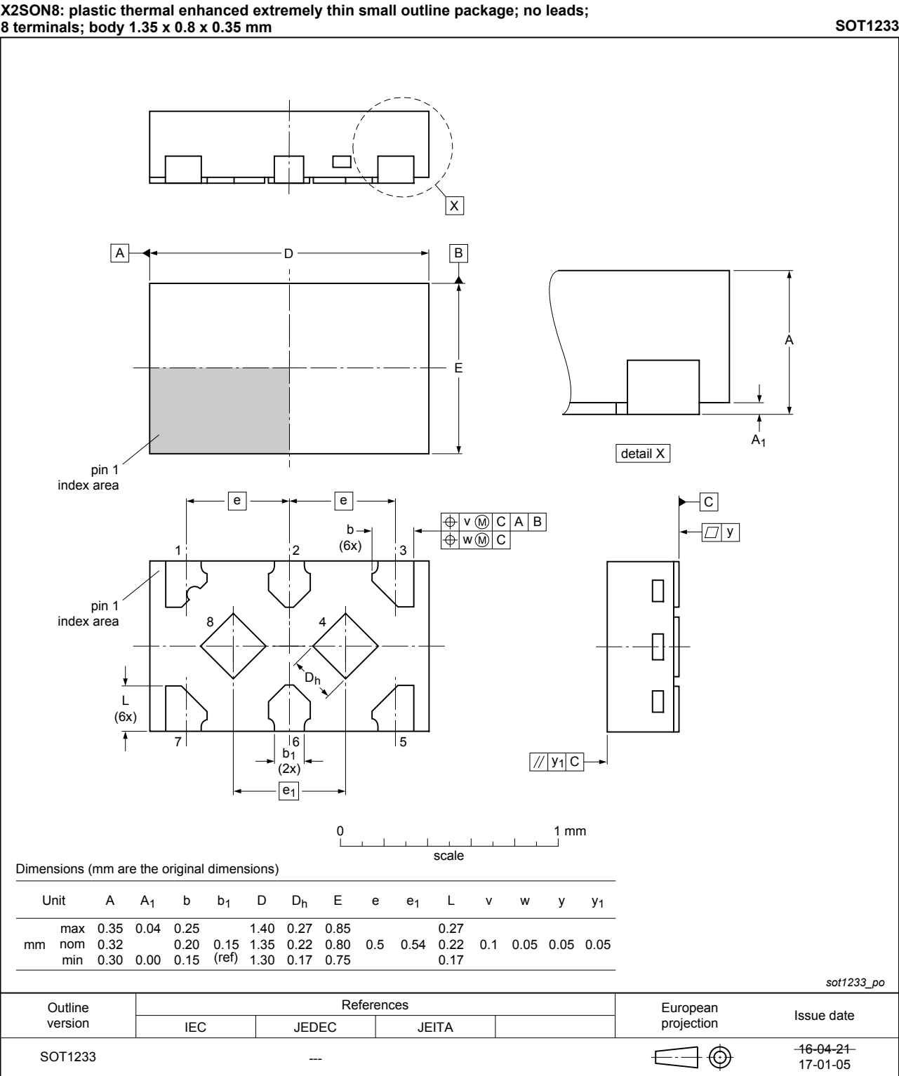
Figure 27. Package outline SOT1233 (X2SON8)
