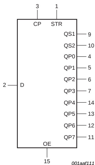
Fig 1. Functional diagram
