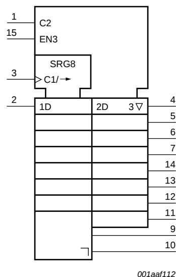
Fig 2. Logic symbol
