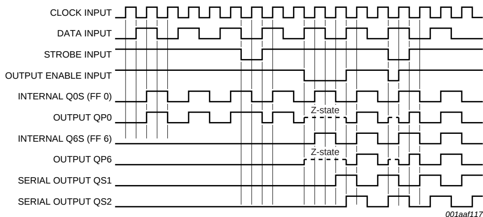
Fig 7. Timing diagram
