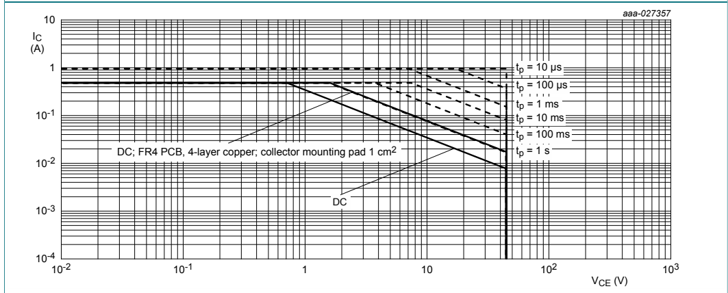
Figure 2. Safe operating area; junction to ambient; continuous and peak collector currents as a function of collector-emitter voltage
