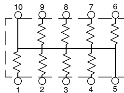
NRSNØ6D8 Circuit Type "D" Bussed/Common
