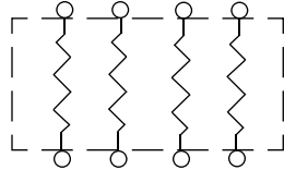
NRSNA4I4/Ø4I NRSNA6I/Ø6I & NRSN12I Circuit Type "I" Isolated
