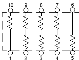
NRSNØ6C8 Circuit Type "C" Bussed/Common
