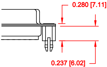
05X ..... 0.237" (BOARD SIDE) - CN10
