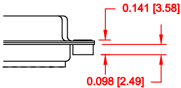
01X ..... 0.098" (BOARD SIDE) - CN1
