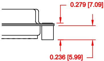
02X ..... 0.236" (BOARD SIDE) - CN2
