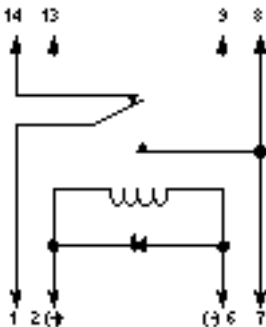
D27F 2 Form A w/Clamp Diode (Top View)
