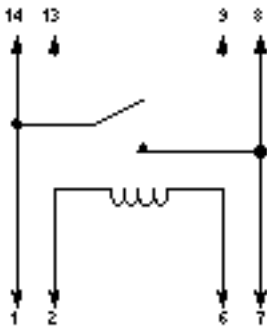
D27G 1 Form B (Top View)
