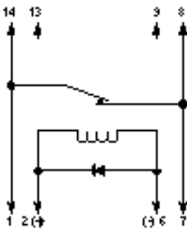
D27H 1 Form B w/Clamp Diode (Top View)
