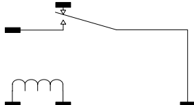
SPDT, 1 Form "C"
