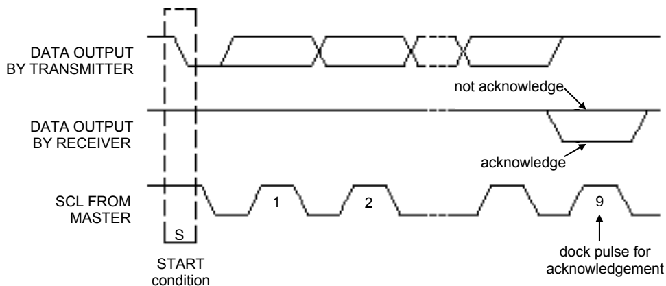
Acknowledge on the I²C-bus
