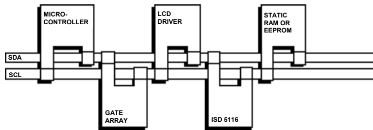
Example of an I²C-bus configuration using two microcontrollers
