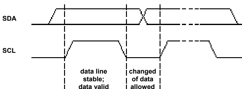
Bit transfer on the I²C-Bus
