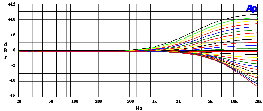
Figure 18: EQ Band 5 Gains for Lowest Cut-Off Frequency
