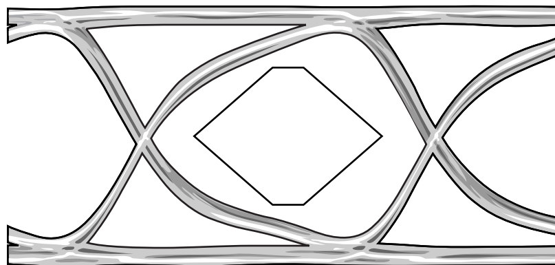
Fig 4. Eye diagram at 2 V receiver common-mode
