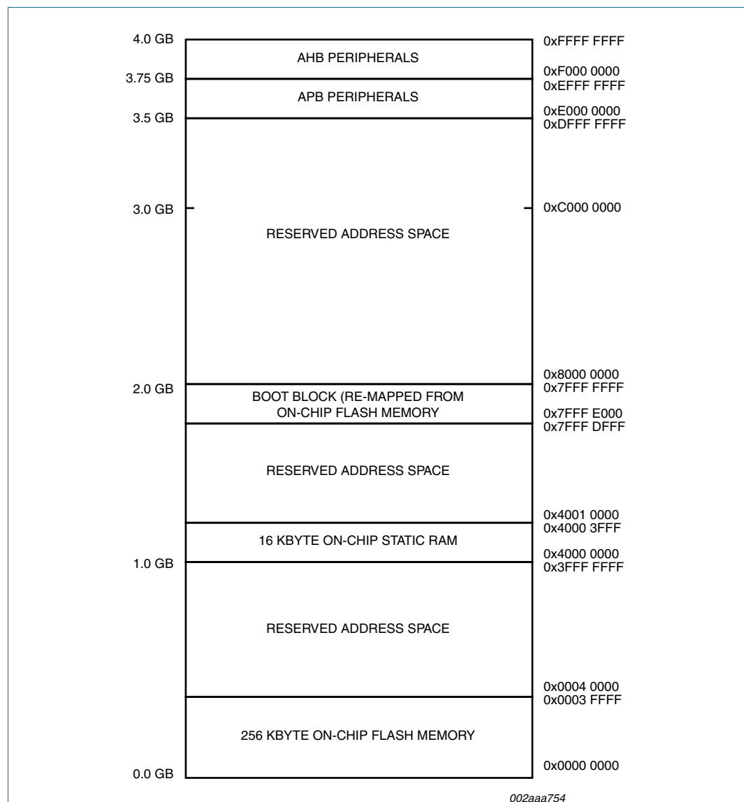
Fig 4. LPC2292/LPC2294 memory map
