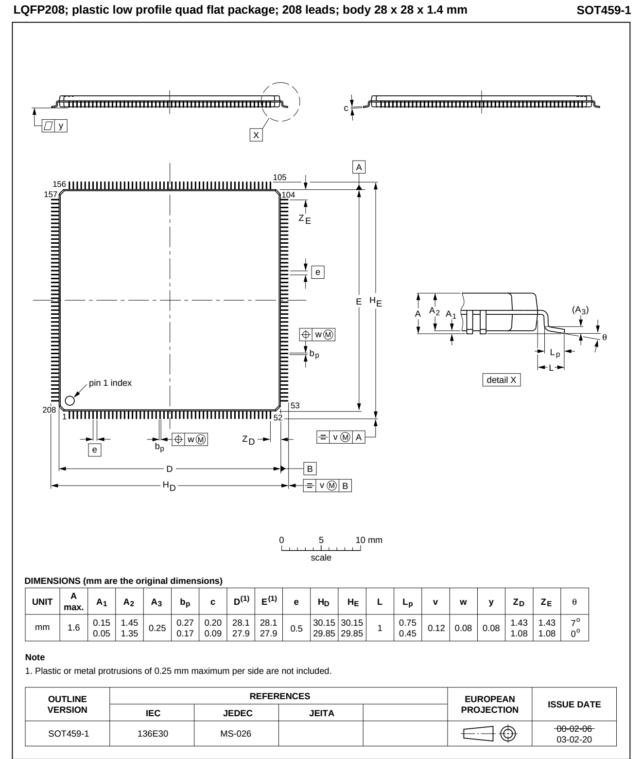
Fig 32. Package outline SOT459-1 (LQFP208)
