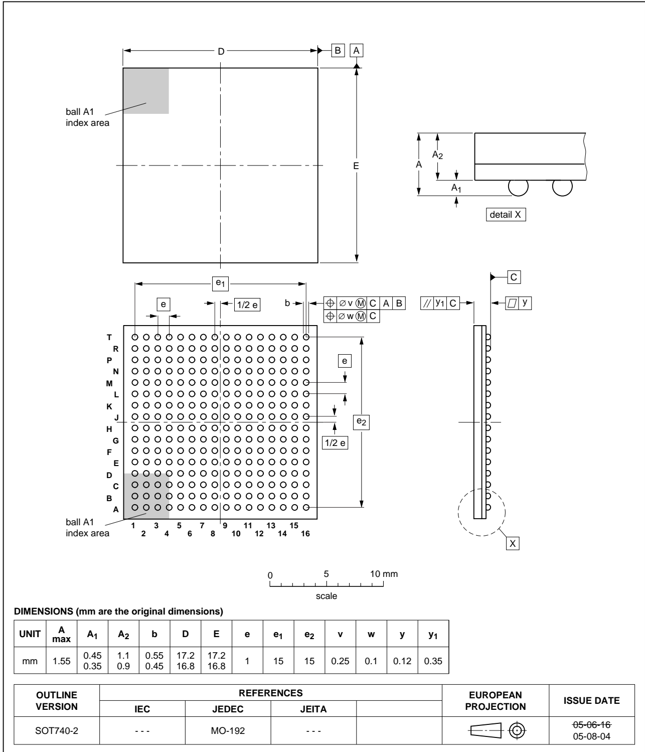
Fig 43. Package outline LPGA256 package
