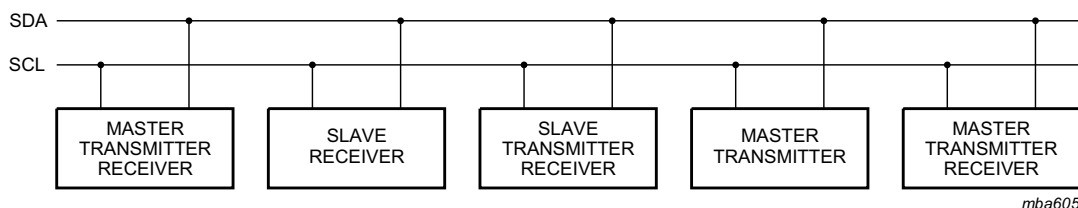
Fig 35. System configuration
