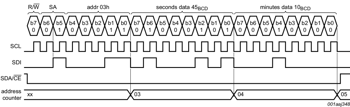
Fig 31. SPI-bus write example
