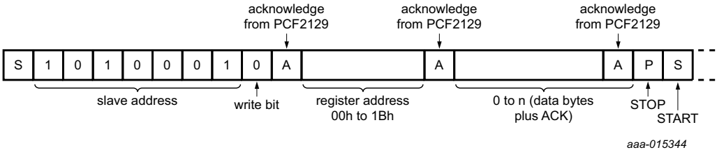
Fig 37. Bus protocol, writing to registers
