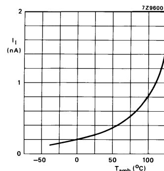
Fig.27 Typical HCMOS input leakage current I_I as a function of ambient temperature T_{\text{amb}} .
