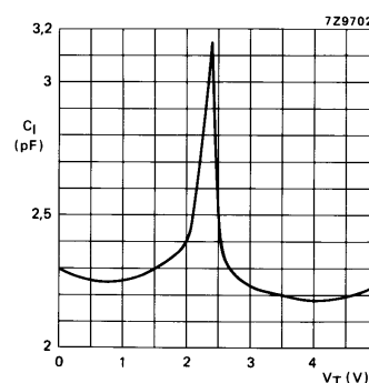
Fig.28 Typical input capacitance C_I of a 74HC device as a function of input voltage; V_{CC} = 5\text{ V} ; T_{\text{amb}} = 25^{\circ}\text{C} .
